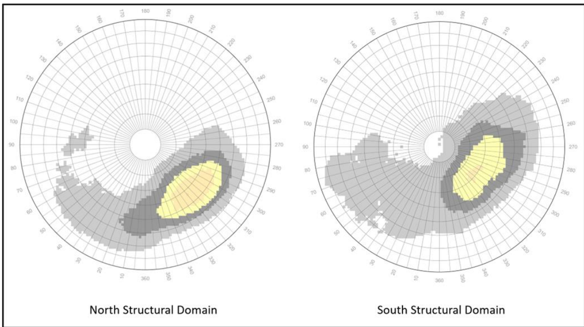
Figure 13-8: North and South Structural Domain Stereonets
