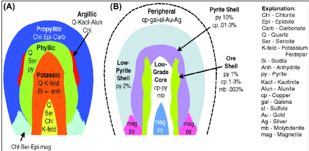
Figure 6-4: Simplified Alteration and Mineralization Zonation Model of a Porphyry Cu Deposit
