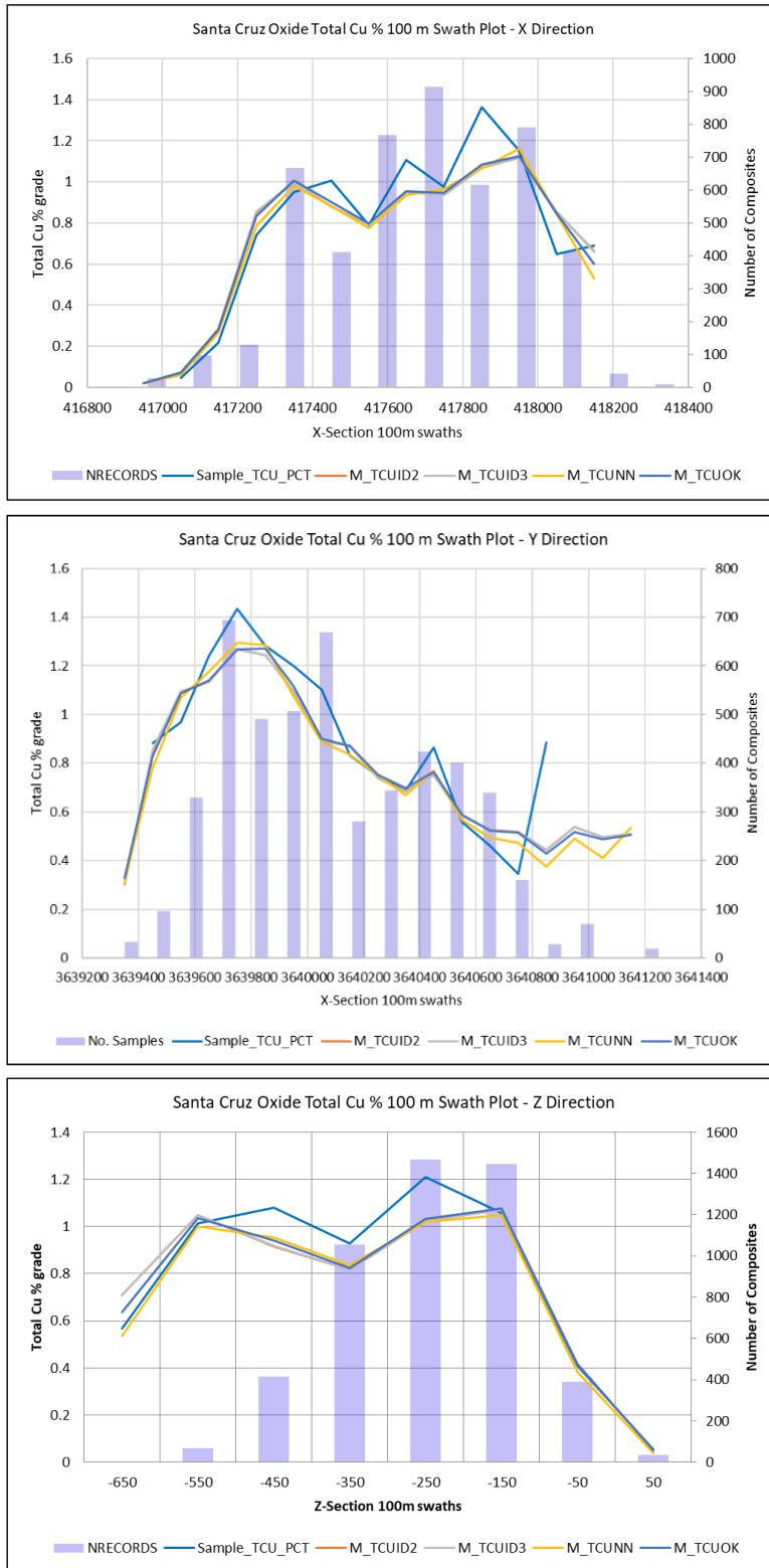
Figure 11-31: Santa Cruz Oxide Domain Swath Plots, Total Cu % in X, Y, and Z Directions
