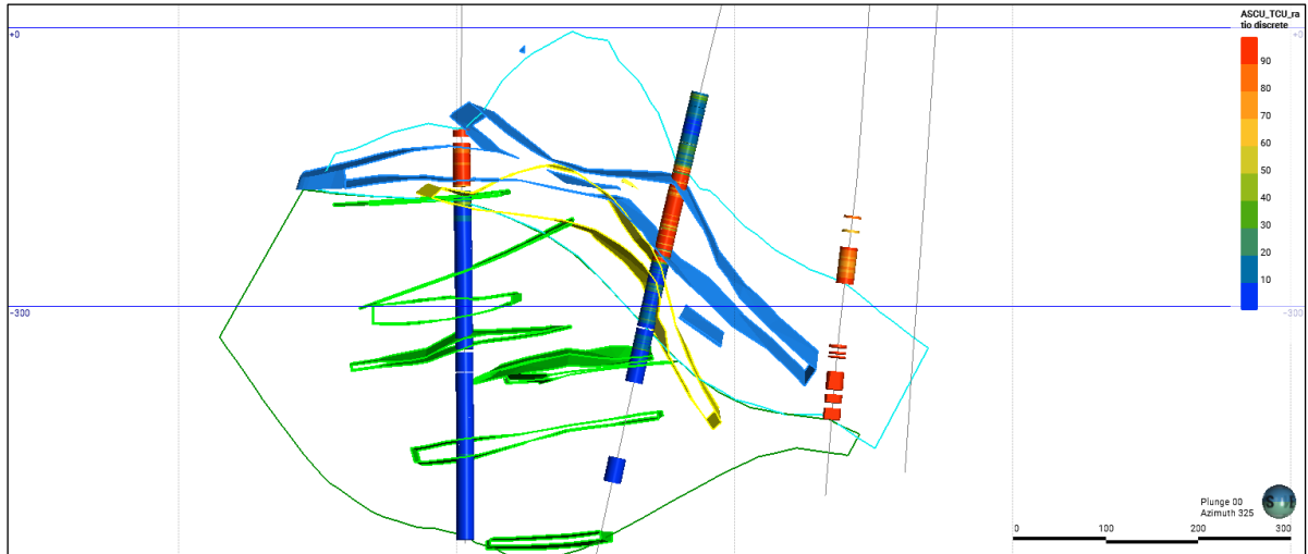
Figure 11-7: Santa Cruz Cross-section Showing Acid Soluble Copper Assay to Total Copper Assay Ratio
