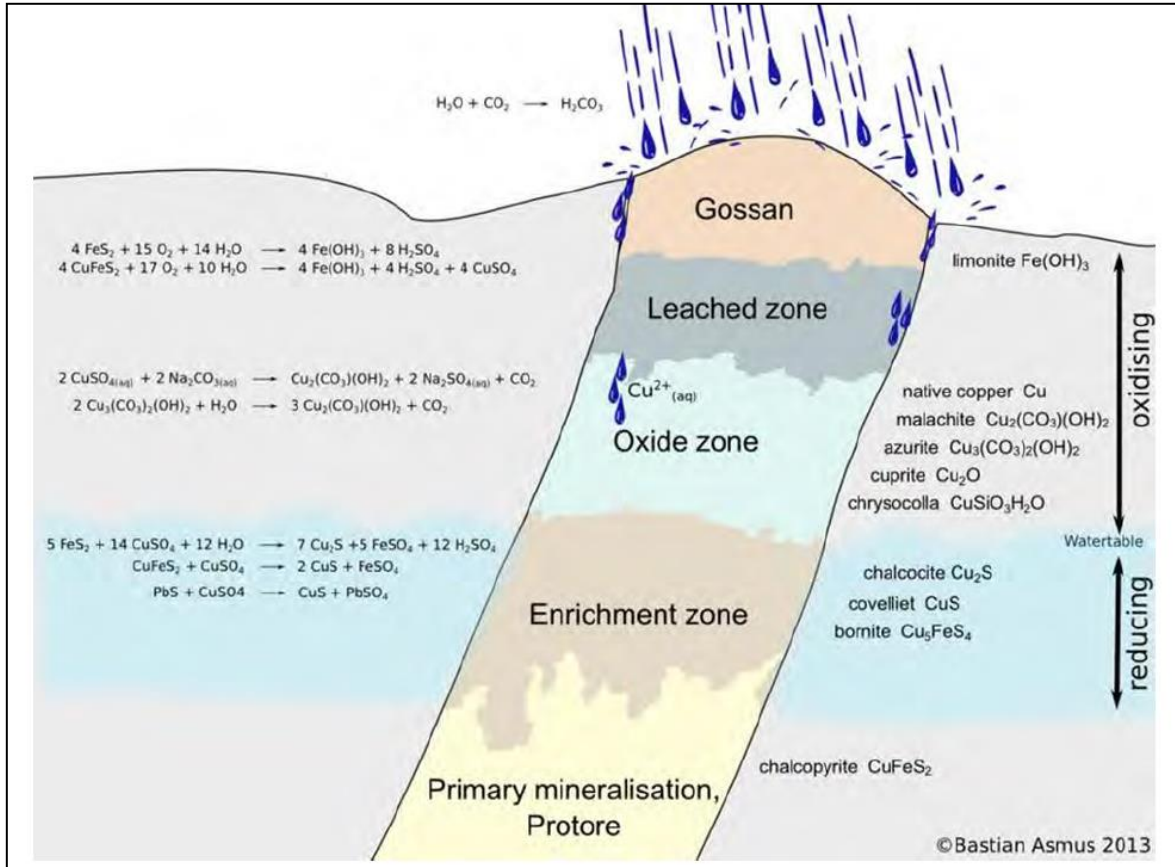
Figure 6-6: Typical Cu Porphyry Cross-section Displaying Hypogene and Supergene Mineralization Processes and Associated Minerals
