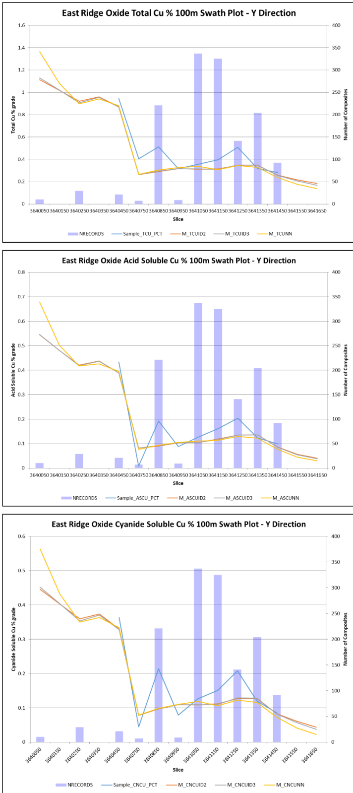
Figure 11-34: East Ridge Oxide Domain Total Cu, Acid Soluble, and Cyanide Soluble Swath Plots
