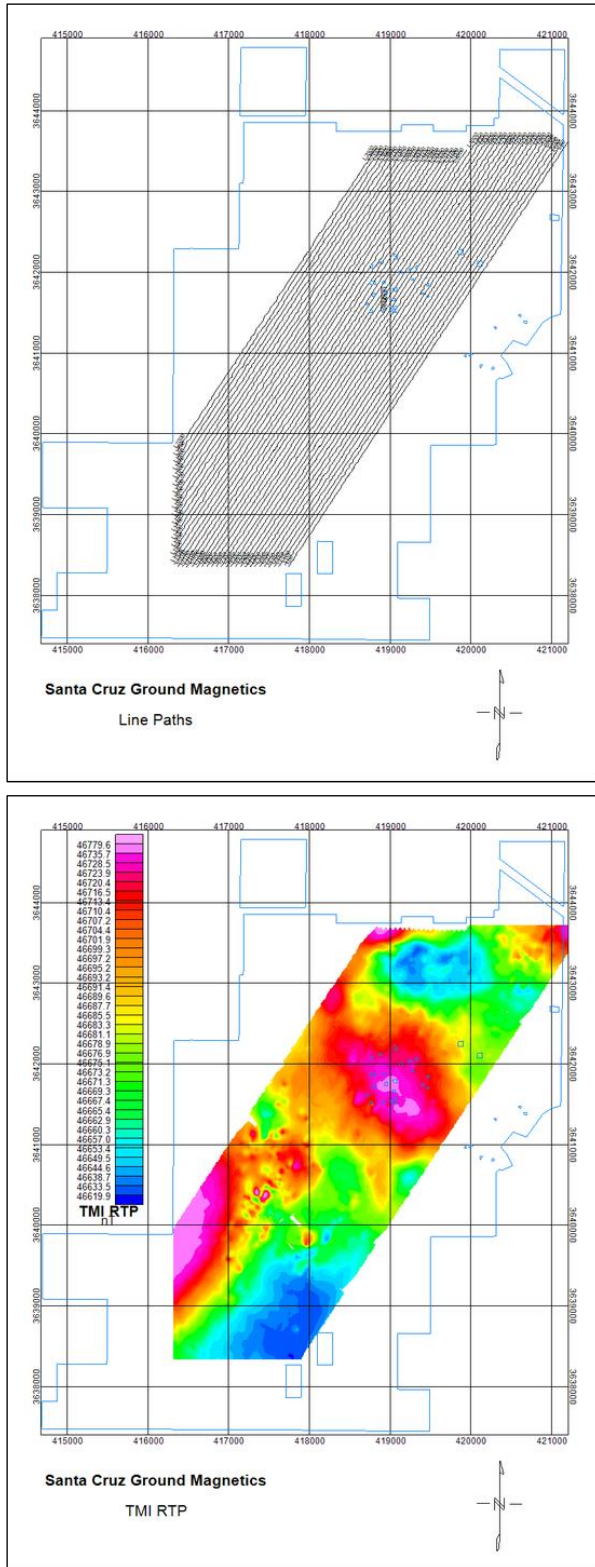
Figure 7-2: Ground Magnetics Survey Lines (top) and Ground TMI RTP Ground Magnetics Results (bottom)
