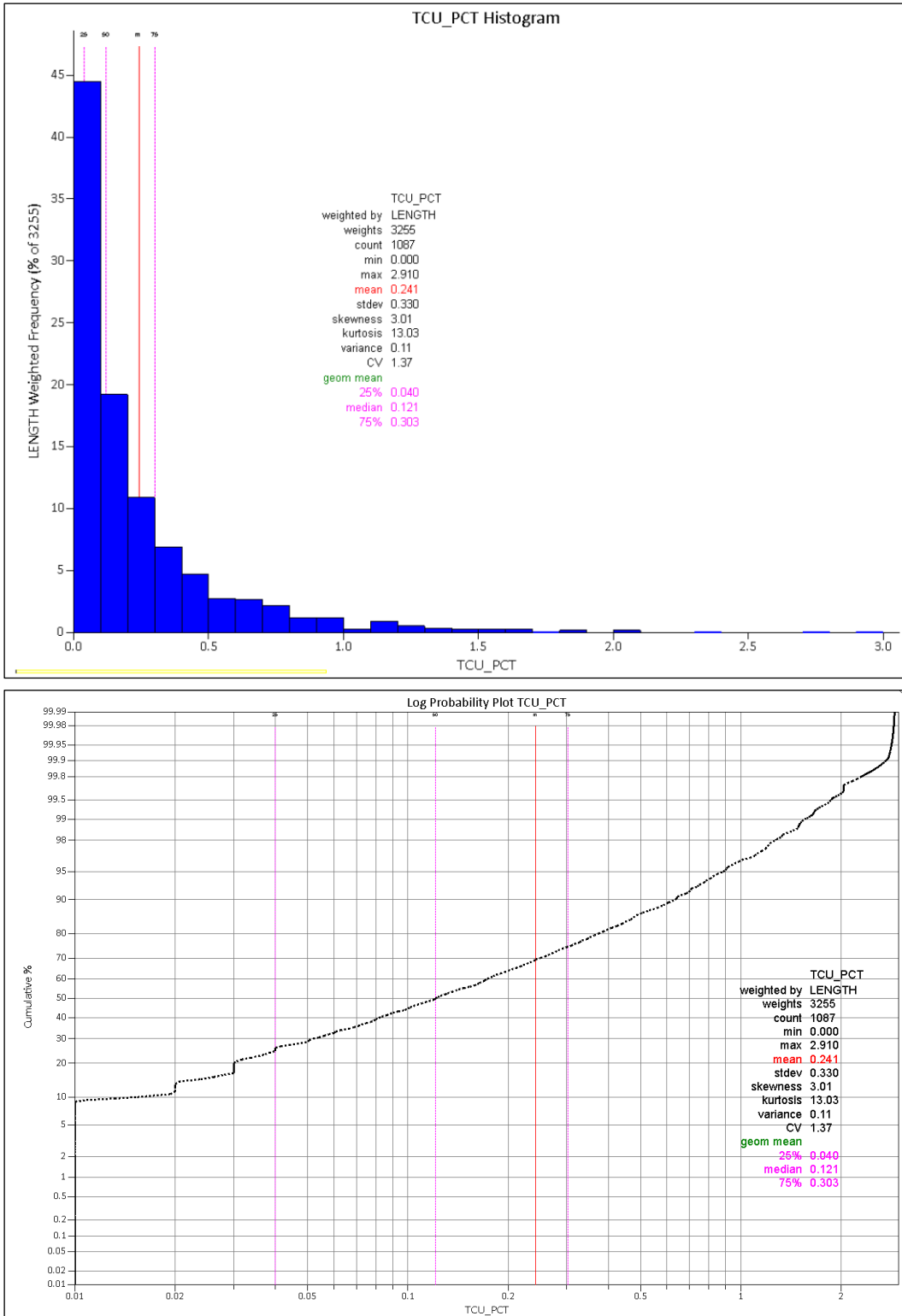
Figure 11-13: Histogram and Log Probability Plots for East Ridge Oxide Cu LG Sub-Domain
