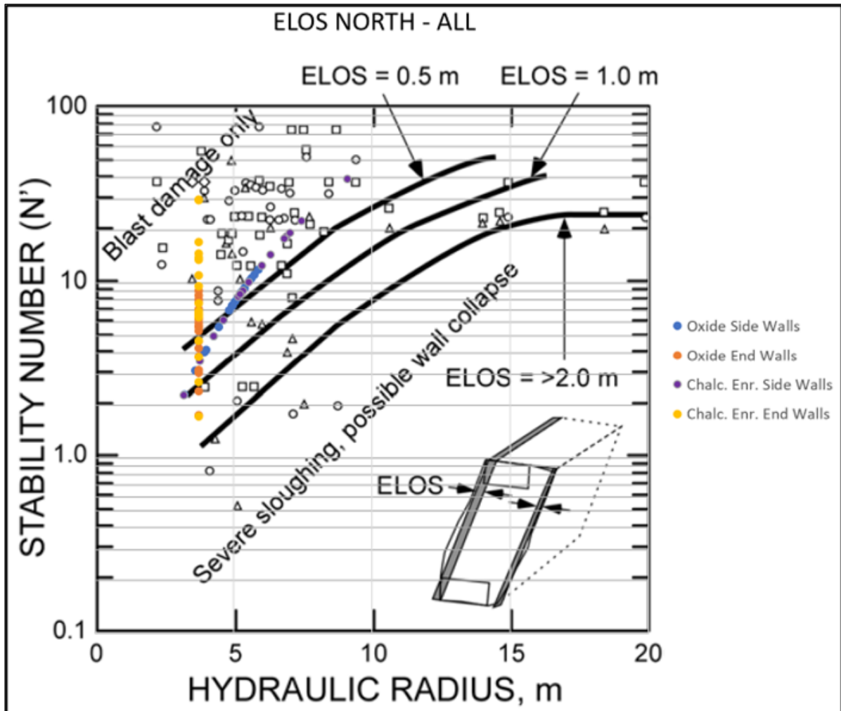
Figure 13-13: North Domain ELOS Estimates (10 m Wide, 30 m High)
