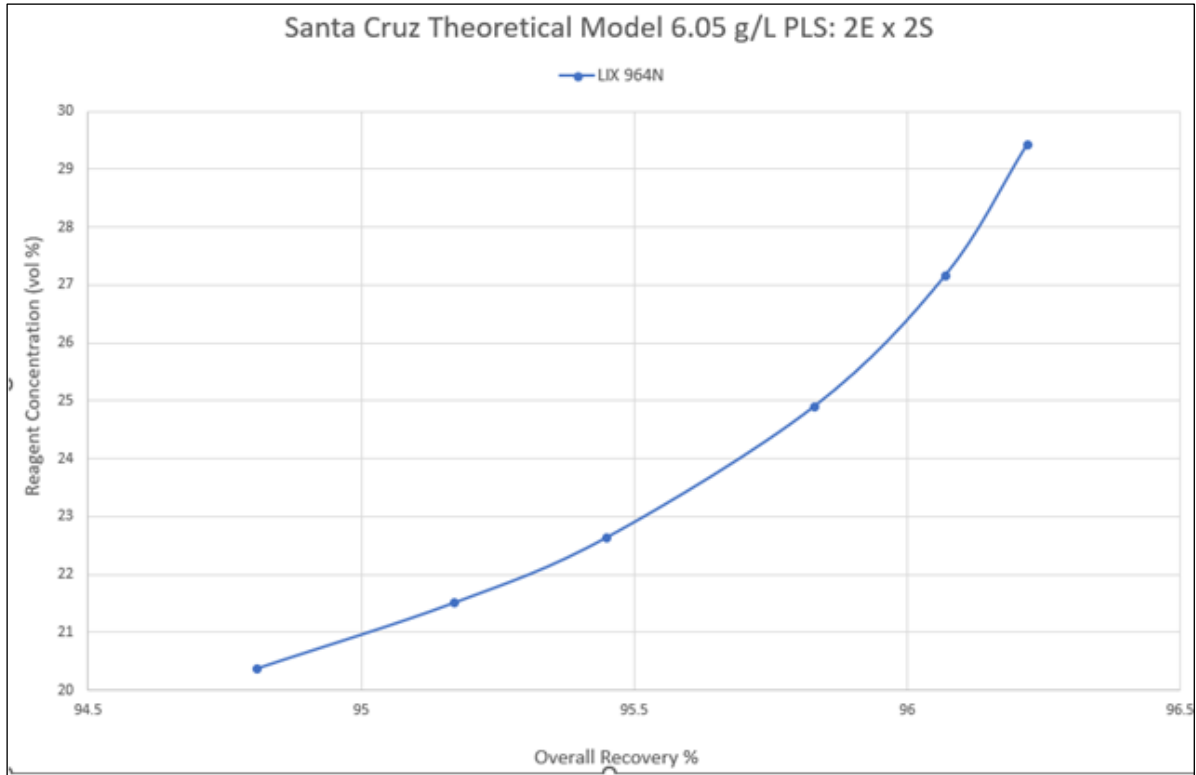
Figure 10-5: Copper Recovery vs Organic Extractant Concentration for PLS Extraction of Copper from Santa Cruz PLS
