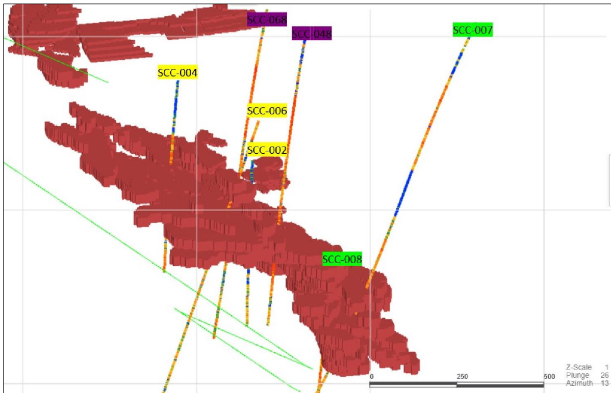
Figure 10-3: Mineral Process Testing Sample Drillhole Intercepts in the Minable Material
