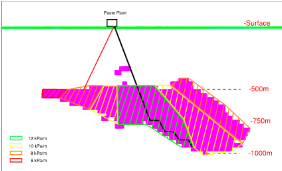
Figure 13-46: Long Section of Paste Distribution System and Maximum Allowable Friction Loss for Gravity Flow (looking East)
