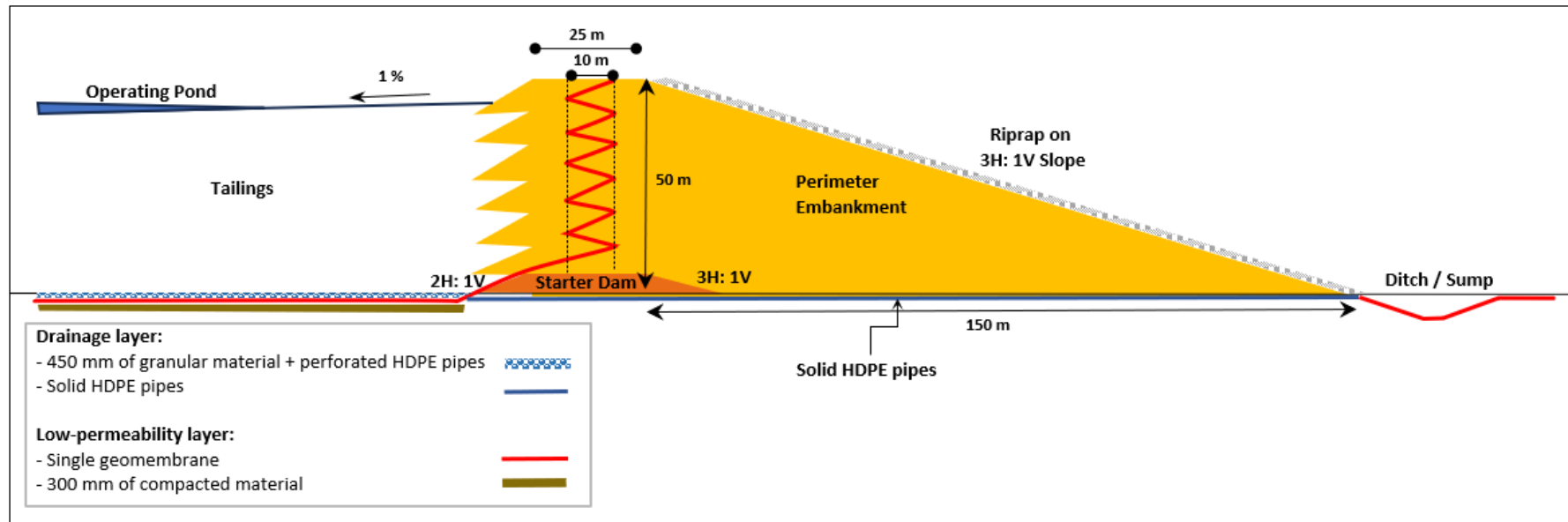
Figure 15-8: TSF Embankment Schematic Cross Section During Operations
