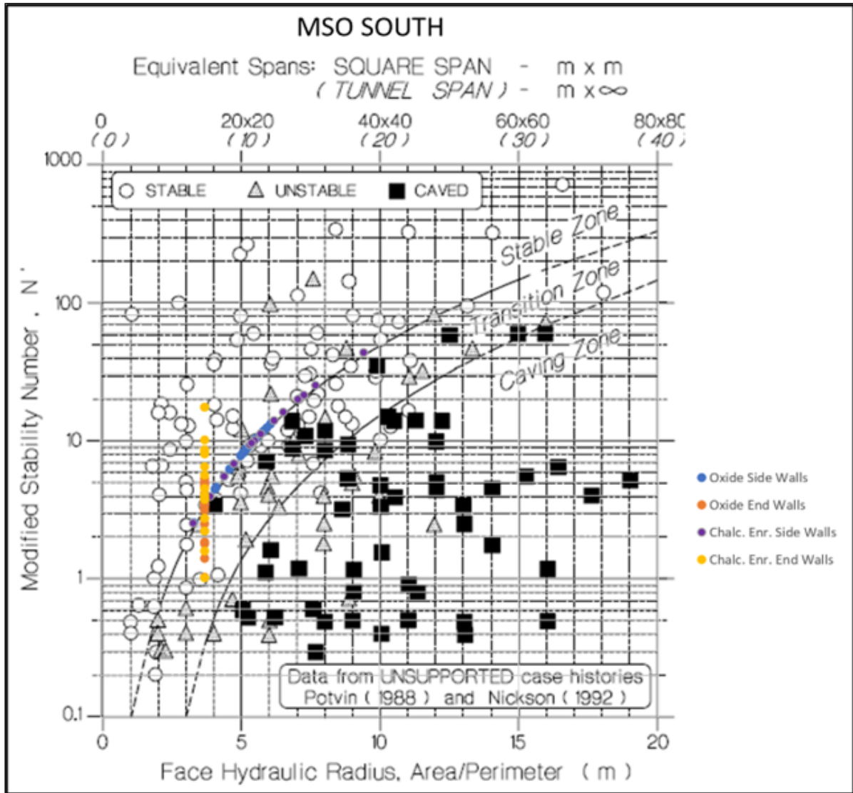
Figure 13-11: South Domain Stability Graph Results (10 m Wide, 30 m High)
