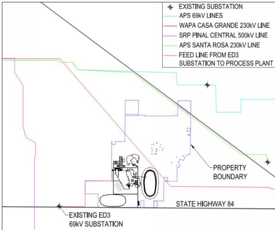
Figure 15-10: Transmission lines near the Santa Cruz Project
