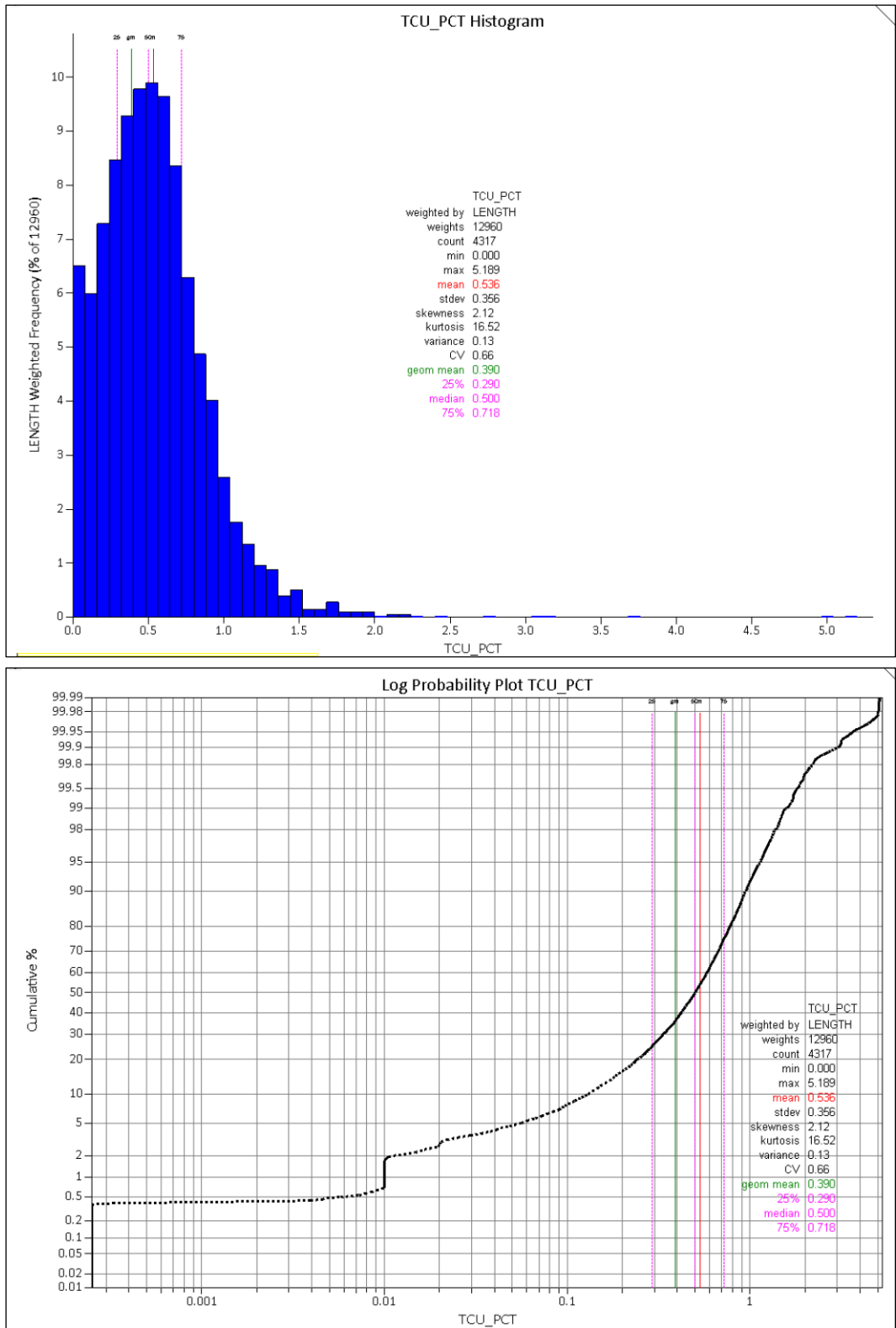
Figure 11-11: Histogram and Log Probability Plots for Santa Cruz Primary Cu LG Sub-Domain
