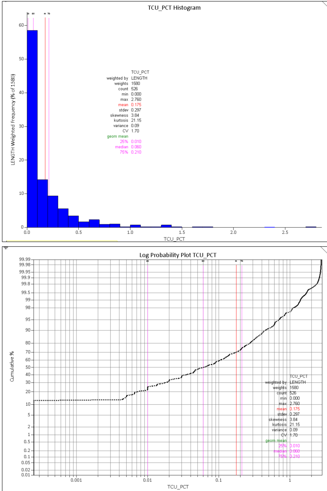
Figure 11-8: Histogram and Log Probability Plots for Santa Cruz Exotic Cu LG Sub-Domain
