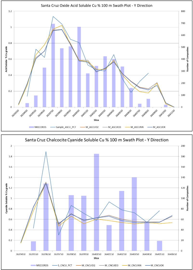
Figure 11-32: Santa Cruz Oxide and Chalcocite Domain Swath Plots, Acid Soluble and Cyanide Soluble Cu %
