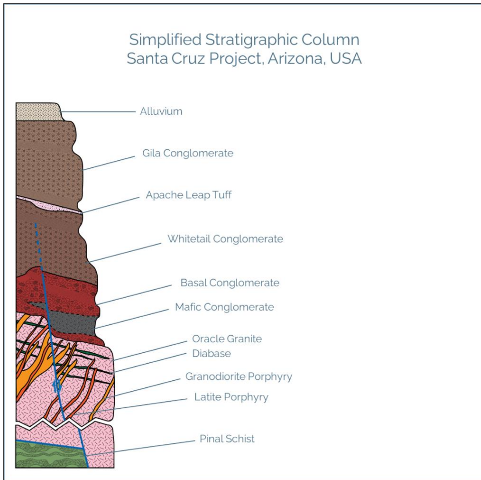
Figure 6-3: Simplified Stratigraphic Section of Santa Cruz Project Alteration
