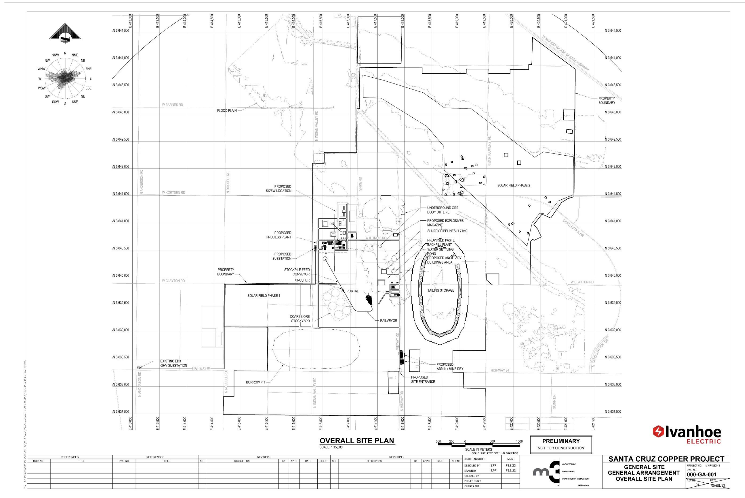
Figure 15-2: Santa Cruz Site Plan
