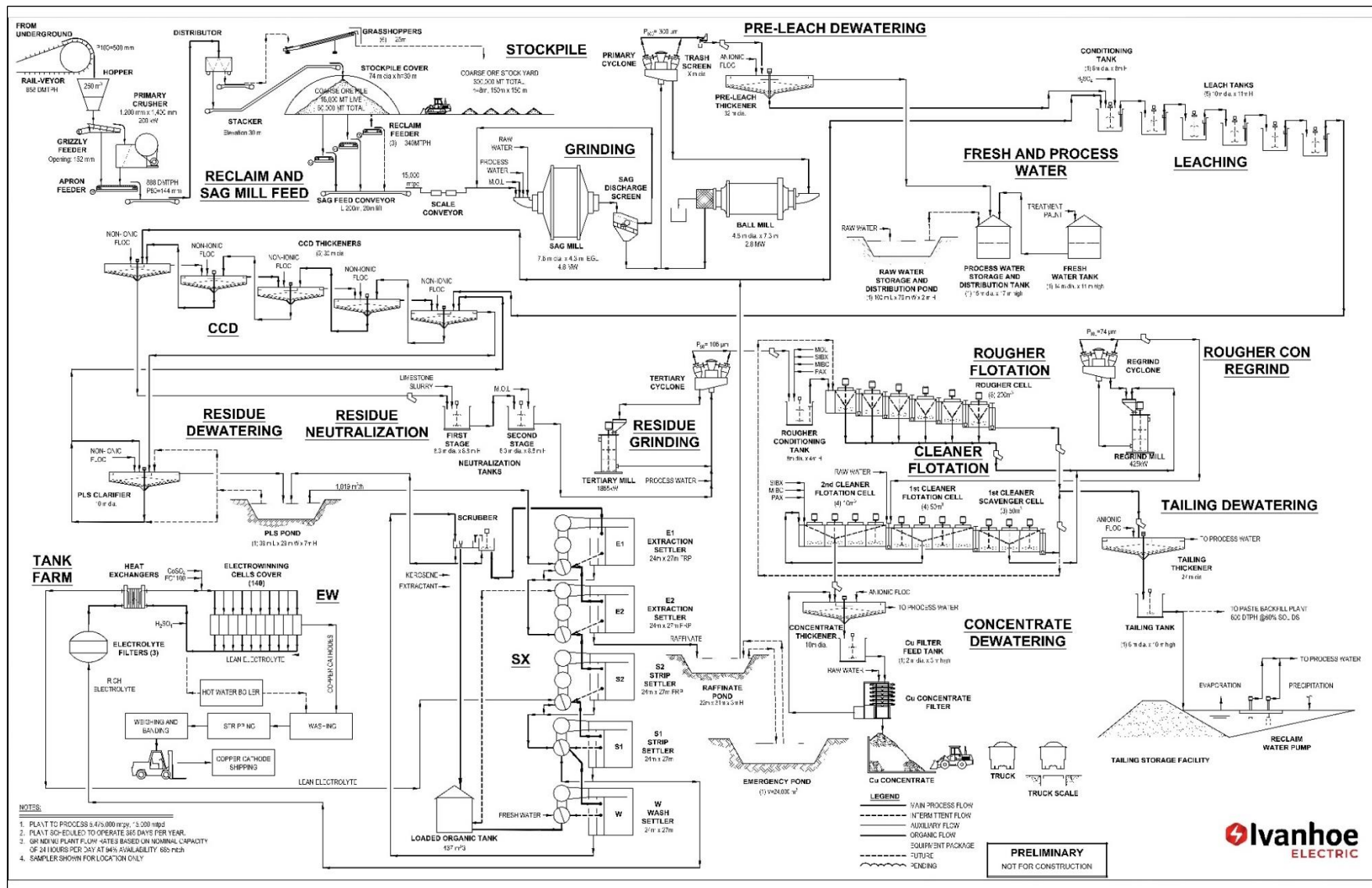
Figure 1-2: Process Flow Sheet
