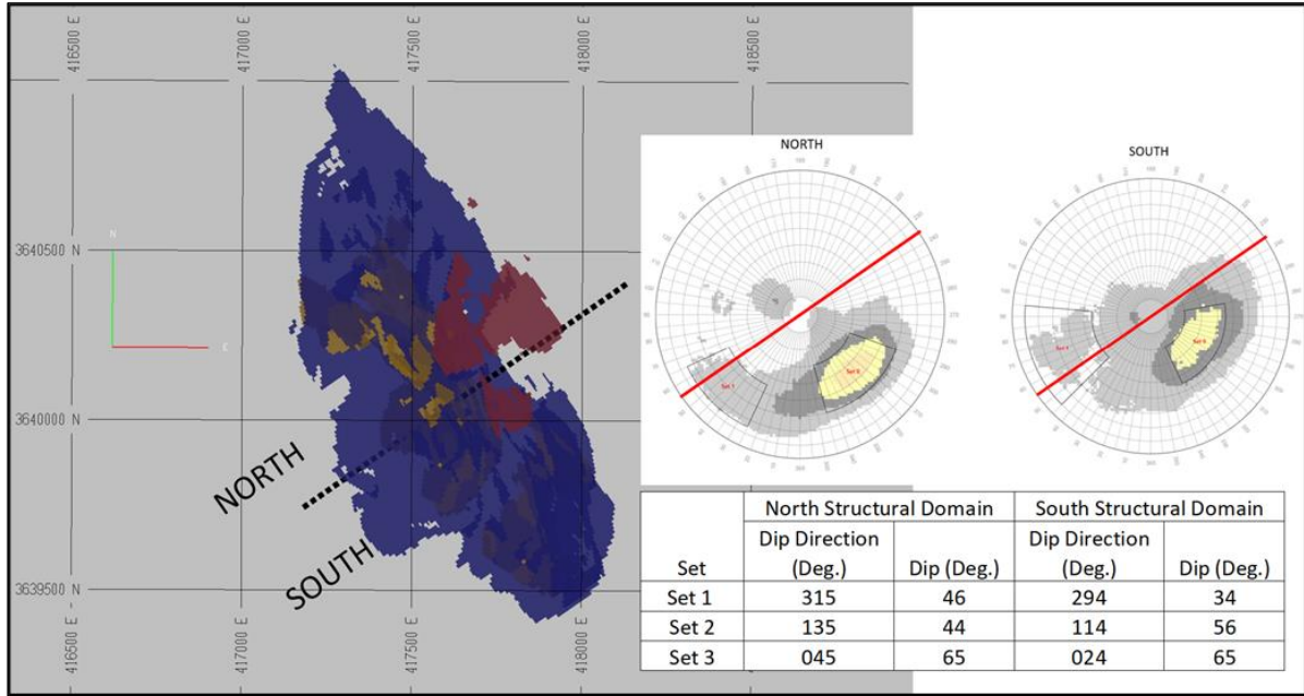
Figure 13-28: Structural Analysis with Dominant Joint Set Orientations
