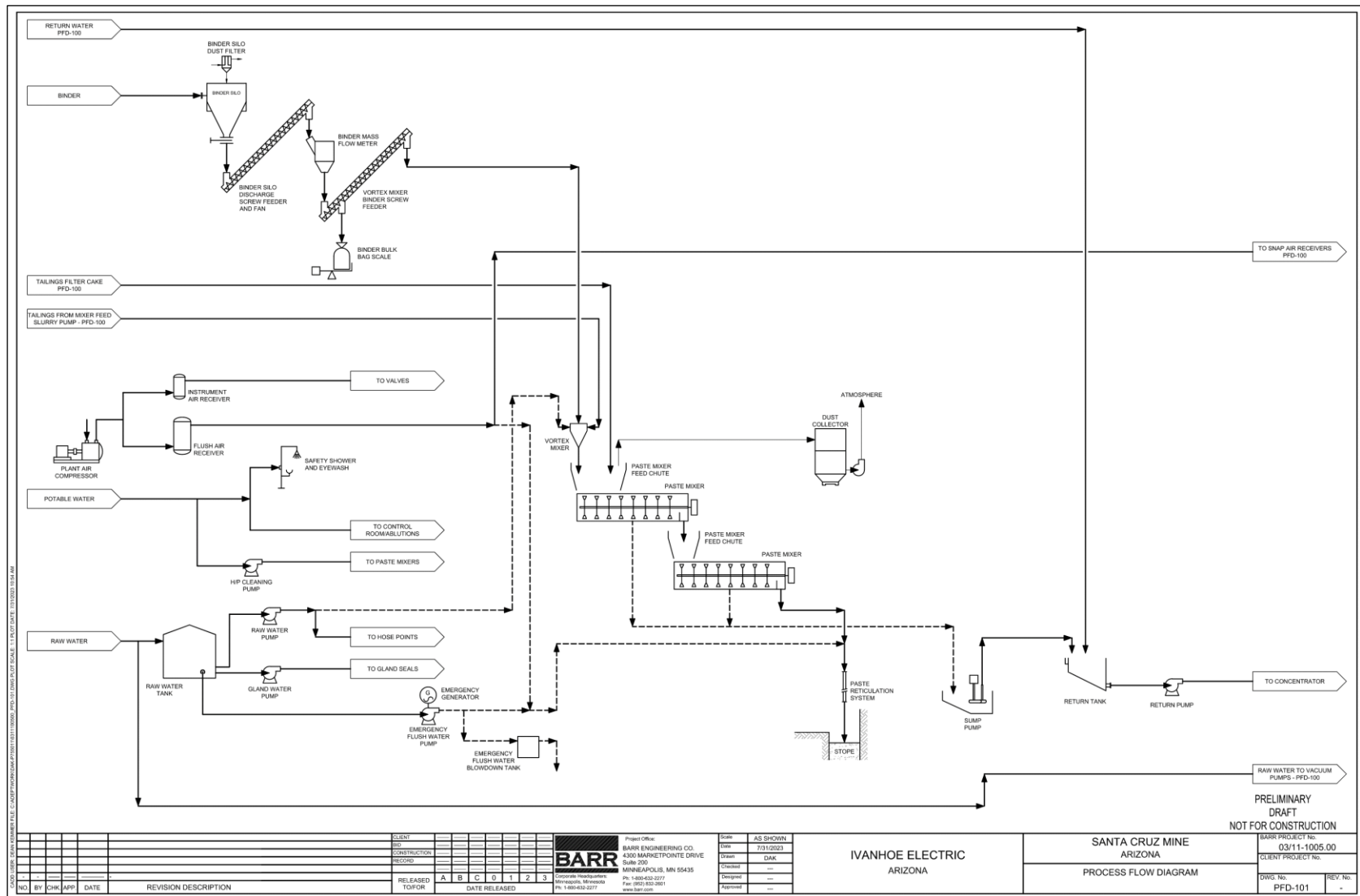
Figure 13-47: Santa Cruz Paste Process Flow Sheet
