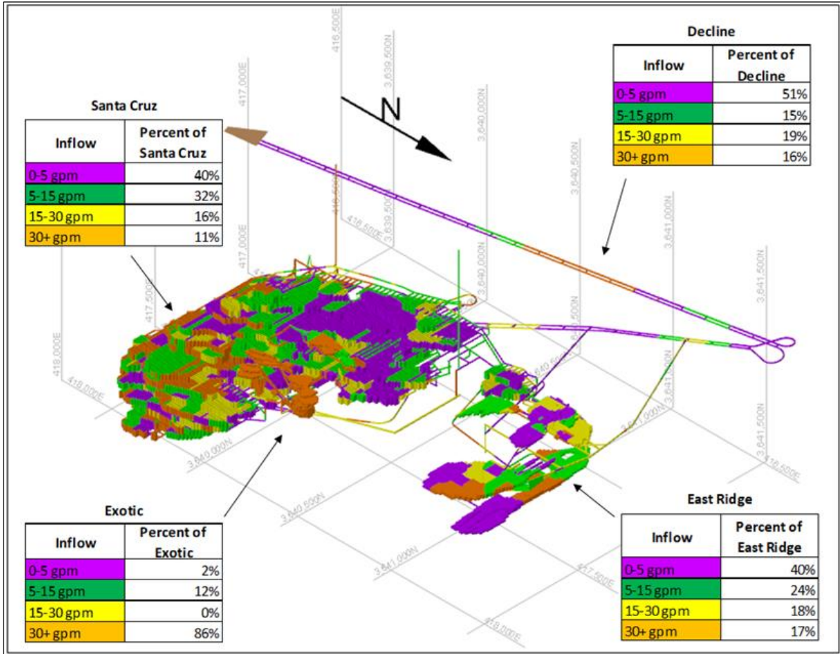
Figure 13-32: Model Estimates of Residual Passive Inflows Mine Workings
