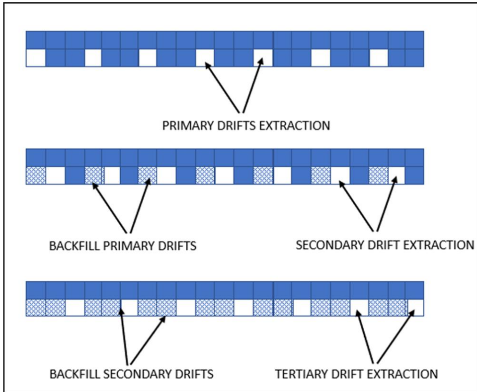
Figure 13-25: PST DAF Mining Sequence
