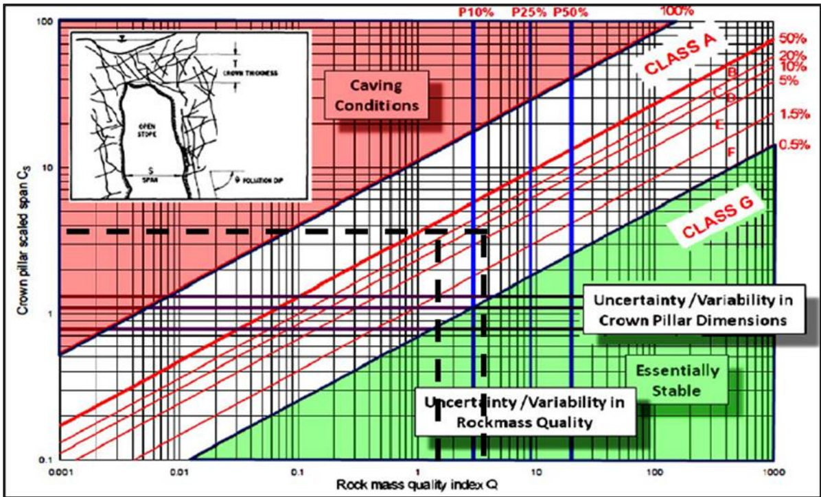
Figure 13-21: Carter's Scaled Span Sill Pillar Estimate
