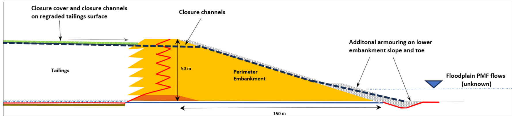
Figure 15-9: TSF Embankment Schematic Cross Section – Closure
