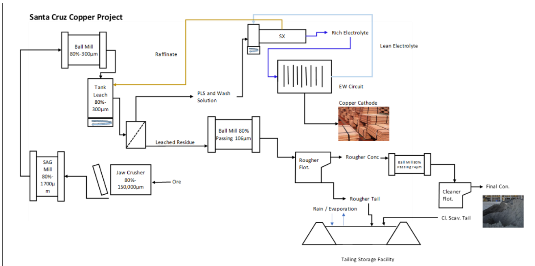
Figure 10-1: Simplified Process Flow Sheet
