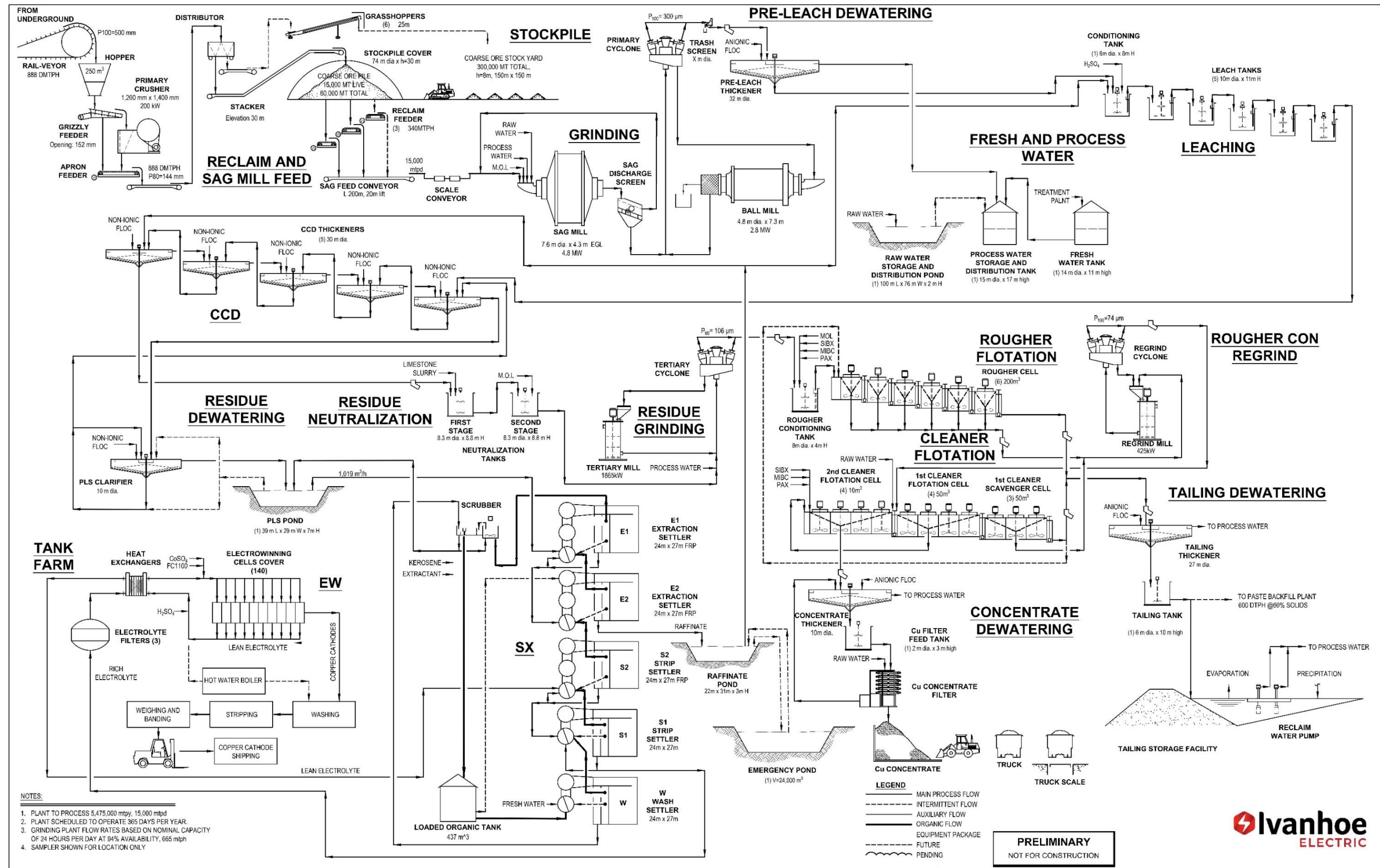
Figure 14-1: Conceptual Flowsheet for the Santa Cruz Process Plant
