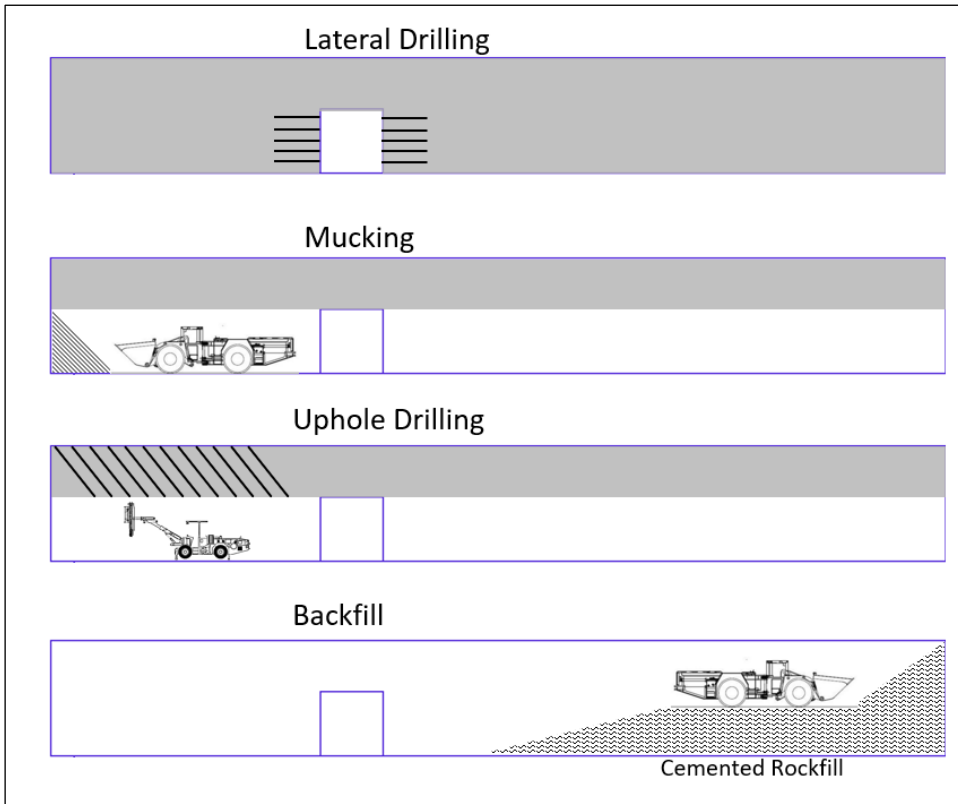
Figure 13-41: Typical Stope Cycle
