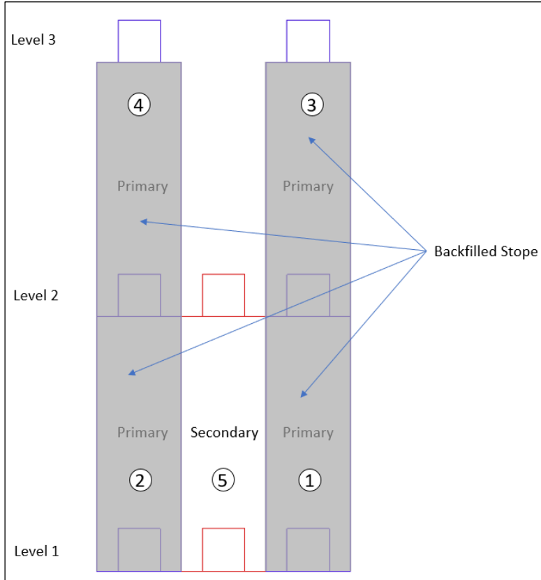
Figure 13-39: Typical Mining Sequence
