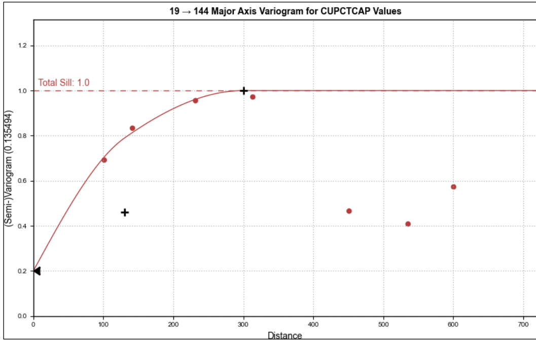
Figure 11-14: Exotic Domain Total Cu Variogram
