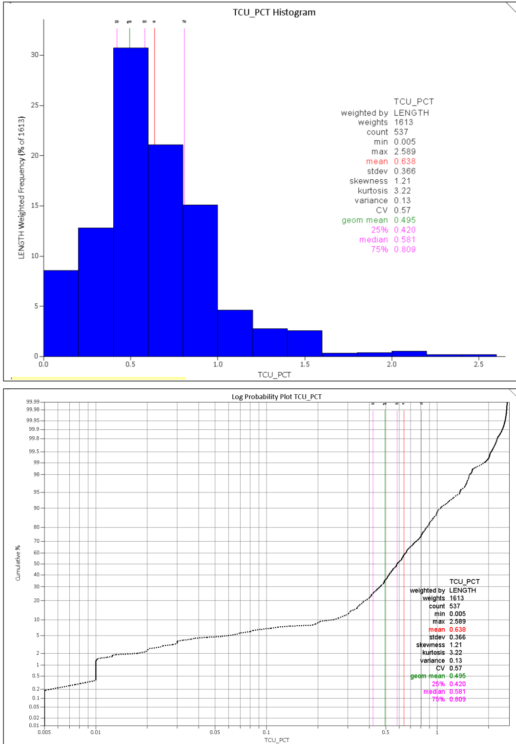
Figure 11-12: Histogram and Log Probability Plots for Texaco Primary Cu LG Sub-Domain
