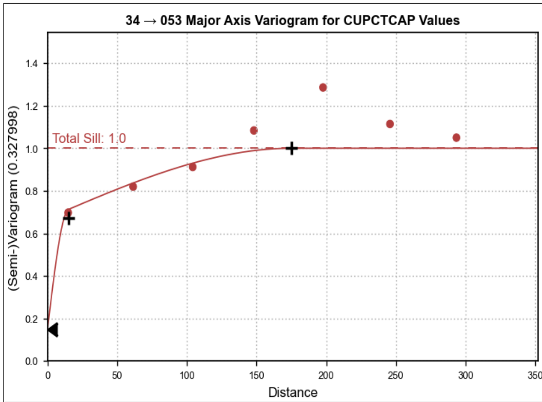
Figure 11-15: Oxide Domain Total Cu Variogram
