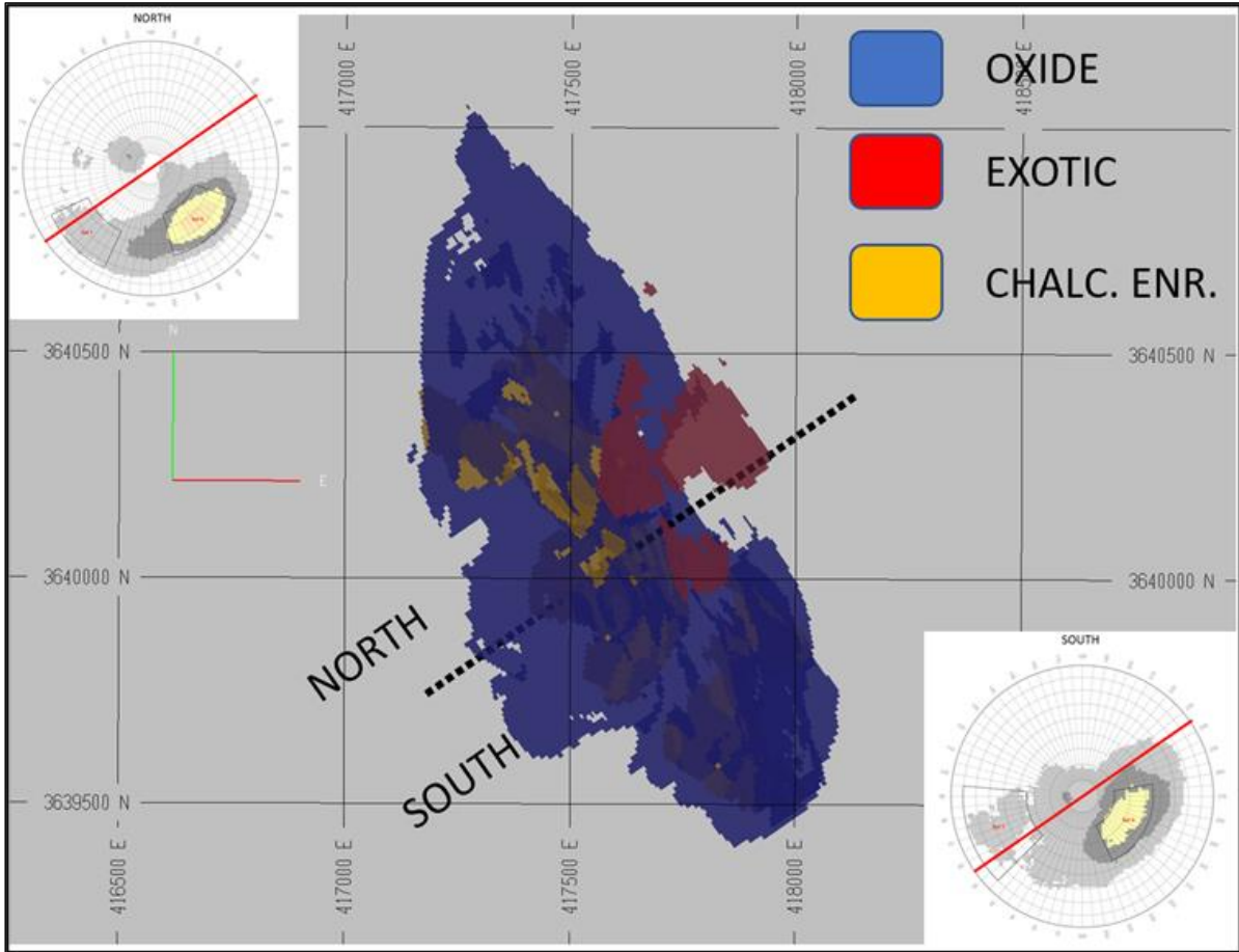
Figure 13-9: North and South Structural Domains
