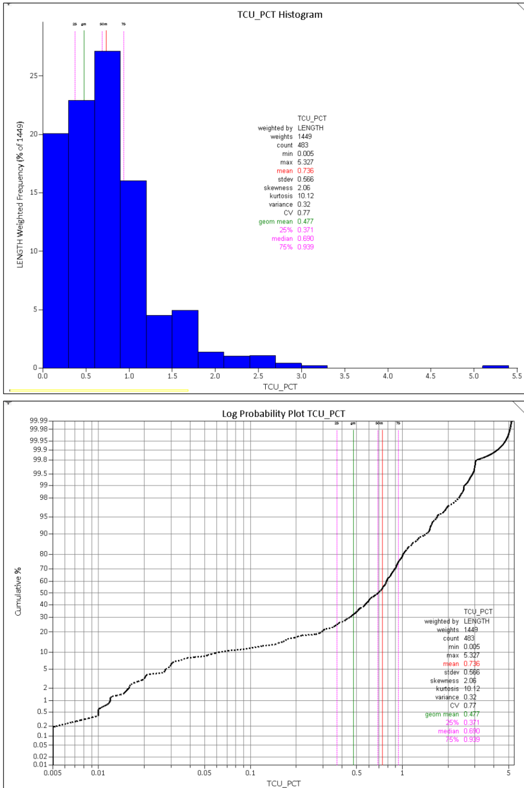
Figure 11-10: Histogram and Log Probability Plots for Santa Cruz Chalcocite Enriched Cu LG Sub-Domain
