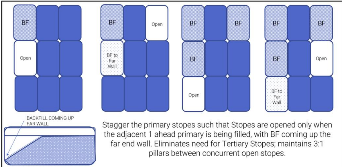
Figure 13-17: Staggered 1-3-5 Sequence Plan View
