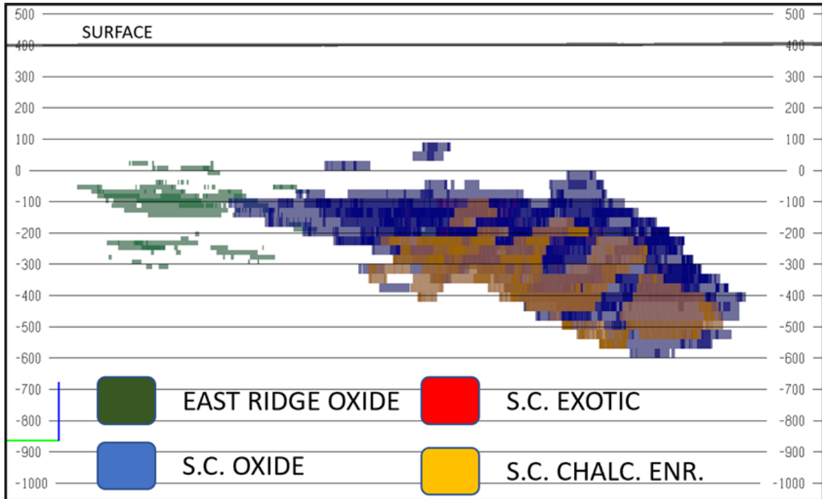
Figure 13-3: Section View (Looking East) of Santa Cruz and East Ridge Mining Targets
