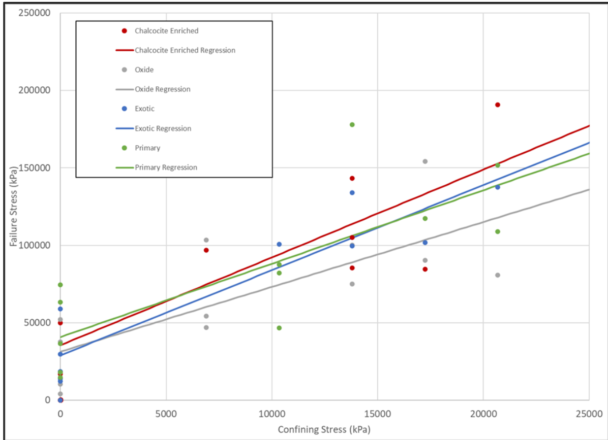
Figure 13-7: Intact Rock Strength Summary
