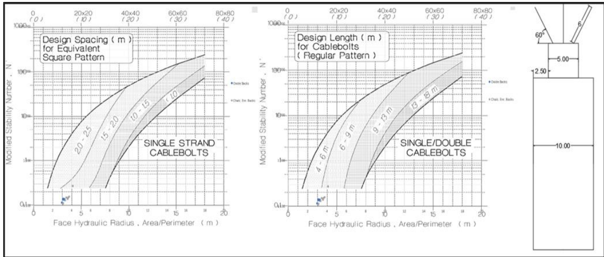
Figure 13-12: Cable Bolt Support
