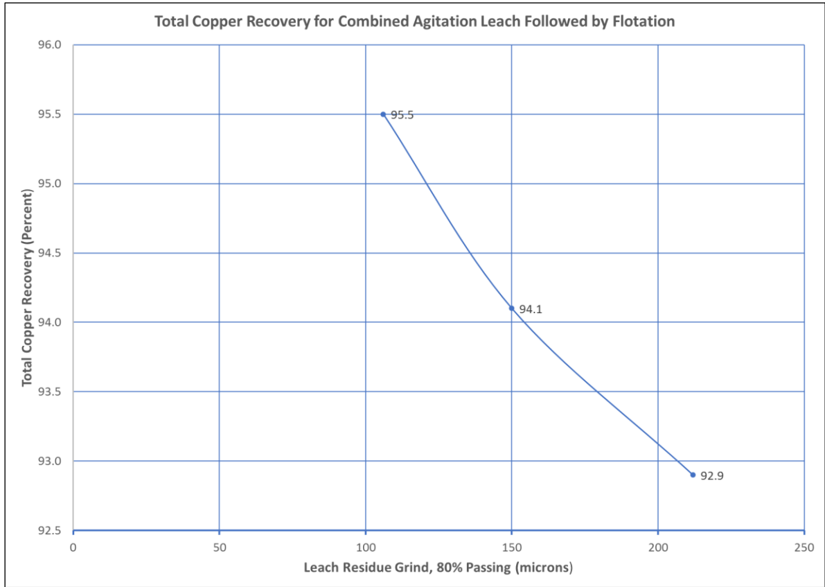
Figure 10-4: Leach – Float Testing Results at Different Leach Residue Grinds
