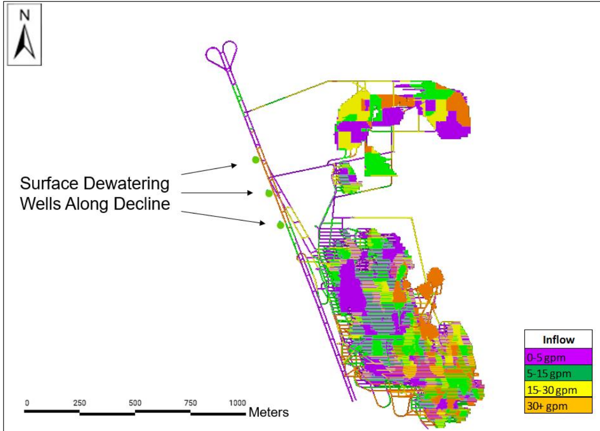
Figure 13-33: Surface Dewatering Well Locations
