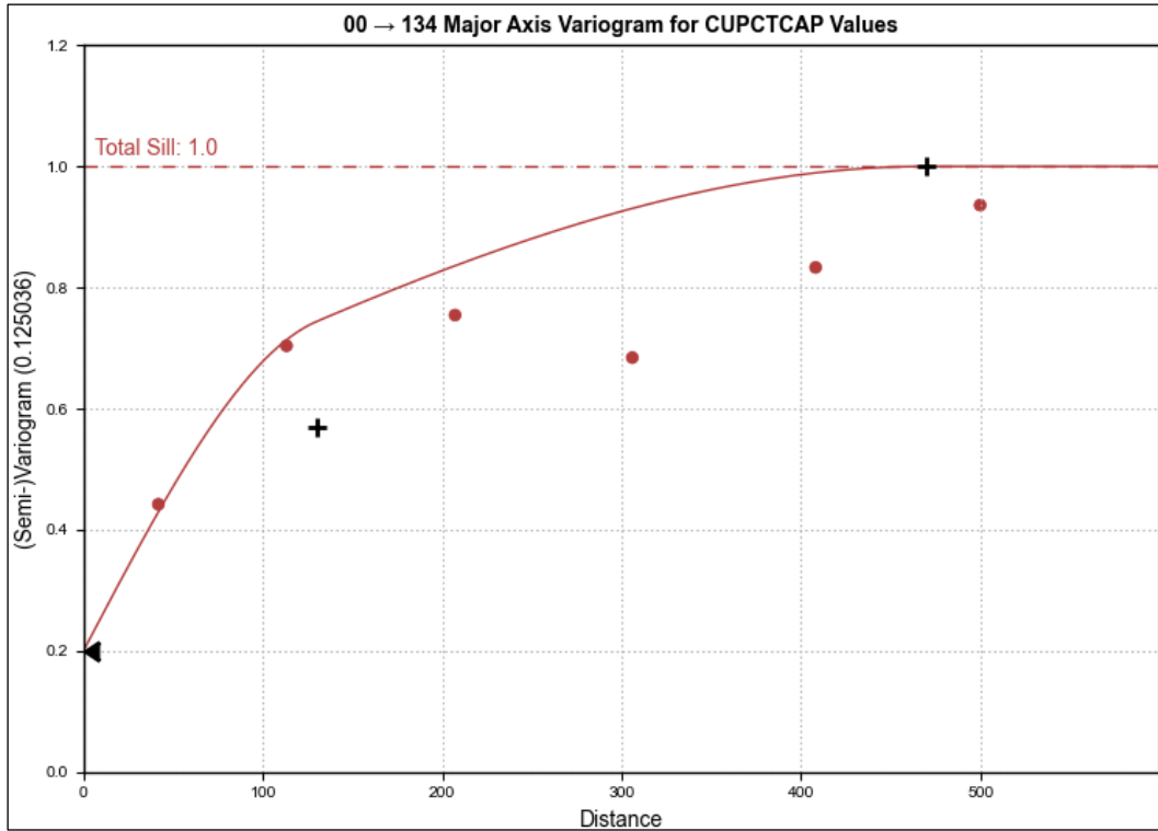
Figure 11-18: Primary Domain Total Cu Variogram
