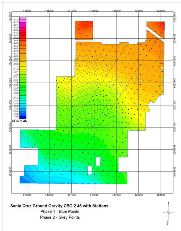
Figure 7-1: Gravity Survey Stations (top) and Complete Gravity Survey Results (bottom)
