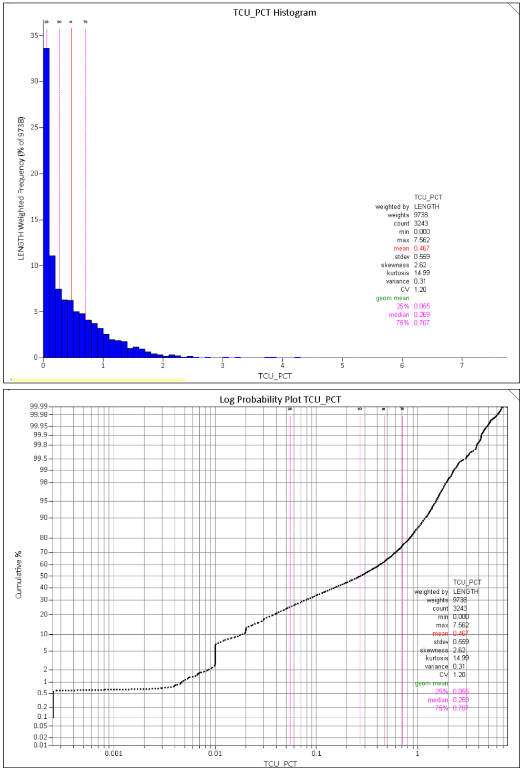
Figure 11-9: Histogram and Log Probability Plots for Santa Cruz Oxide Cu LG Sub-Domain
