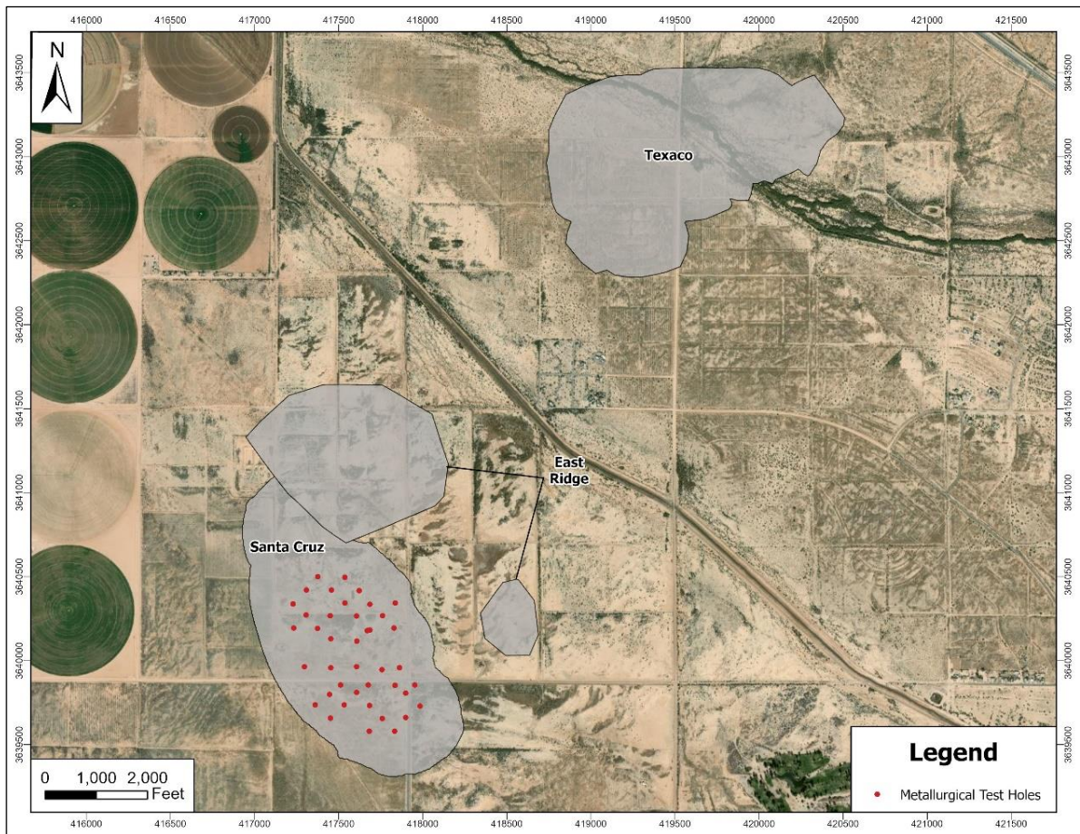
Figure 10-2: Surface Map of the Drillholes Used in the Ore Type Composites
