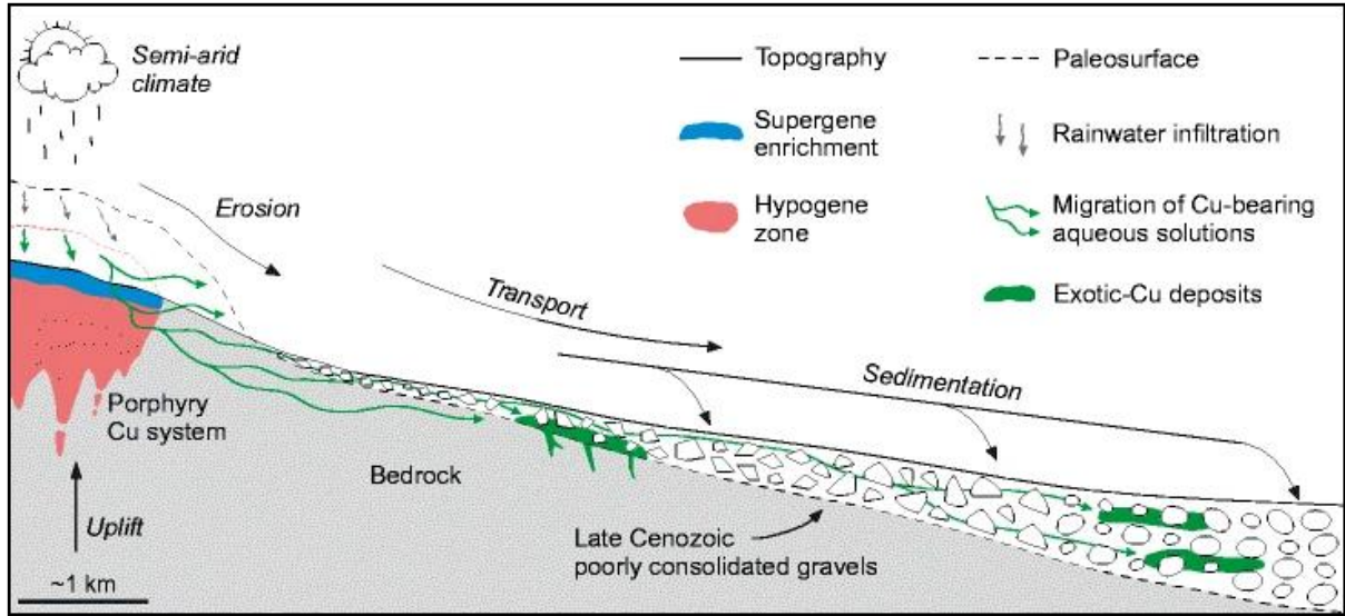
Figure 6-5: Schematic Representation of an Exotic Cu Deposit and its Relative Position to an Exposed Porphyry Cu System
