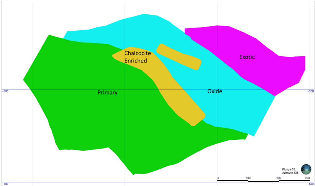
Figure 11-3: Santa Cruz Deposit Domain Idealized Cross-section
