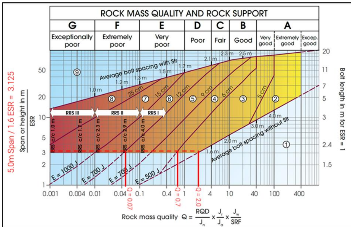
Figure 13-26: Ground Support Category Estimates Using the Ground Support Chart
