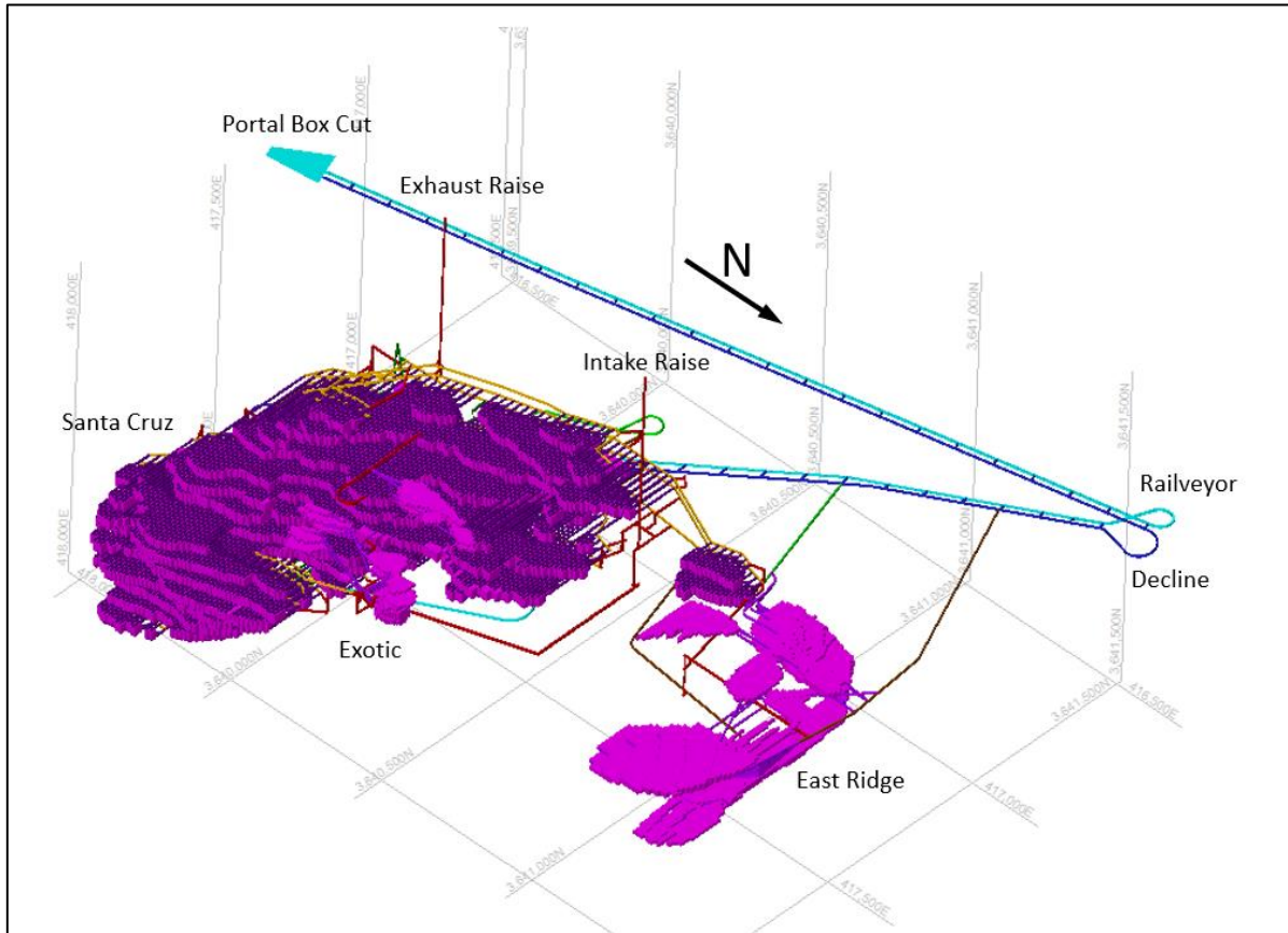
Figure 13-43: Mine Design, Santa Cruz, Santa Cruz Exotic, and East Ridge
