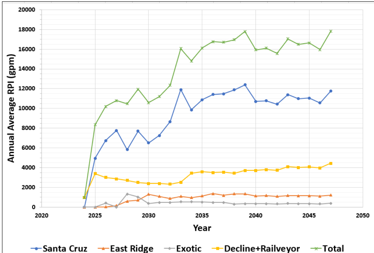
Figure 13-31: Mine Residual Passive Inflow (RPI) by Area and Total Mine Plan Combined with Active Dewatering During Years 1 and 2
