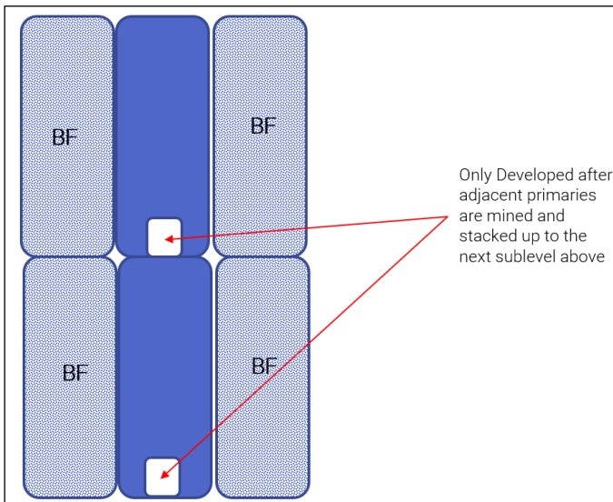
Figure 13-17: Staggered 1-3-5 Sequence Plan View
