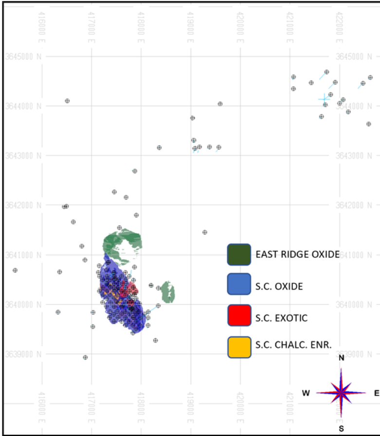
Figure 13-4: Plan View of Geotechnical Drillhole Collars
