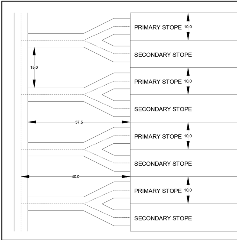
Figure 13-19: Haulage Setback Minimum Distances
