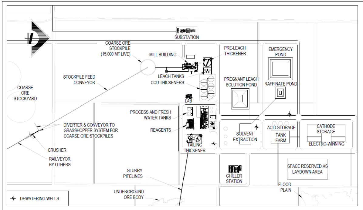
Figure 14-2: Conceptual Santa Cruz Plant Layout
