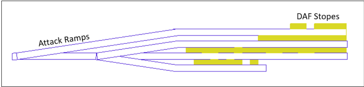
Figure 13-40: Attack Ramp Access to Stopes
