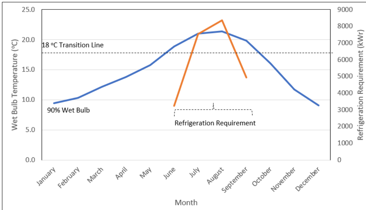
Figure 13-50: Seasonal Refrigeration Operation
