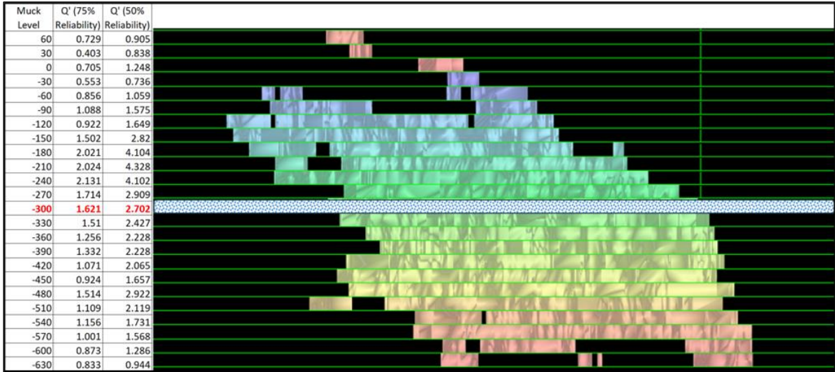
Figure 13-20: Proposed Sill Pillar
