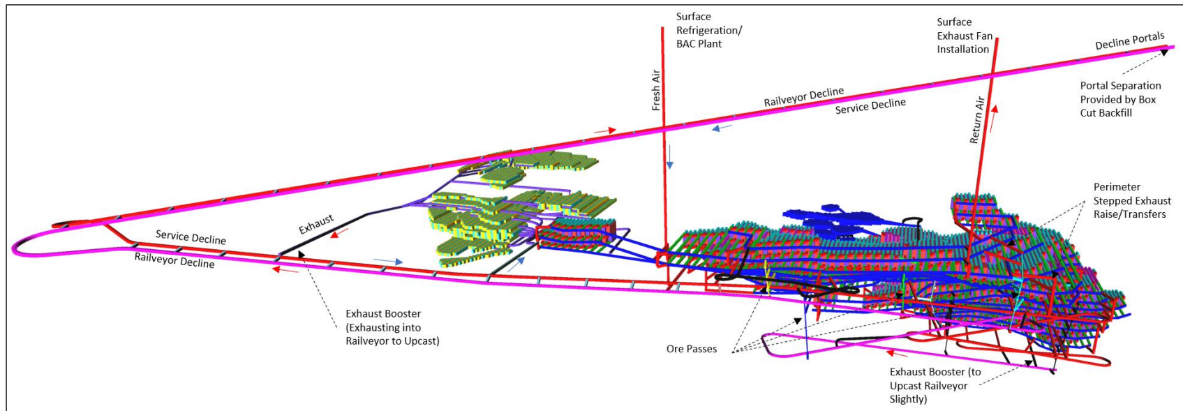
Figure 13-48: General Ventilation Infrastructure and Layout
