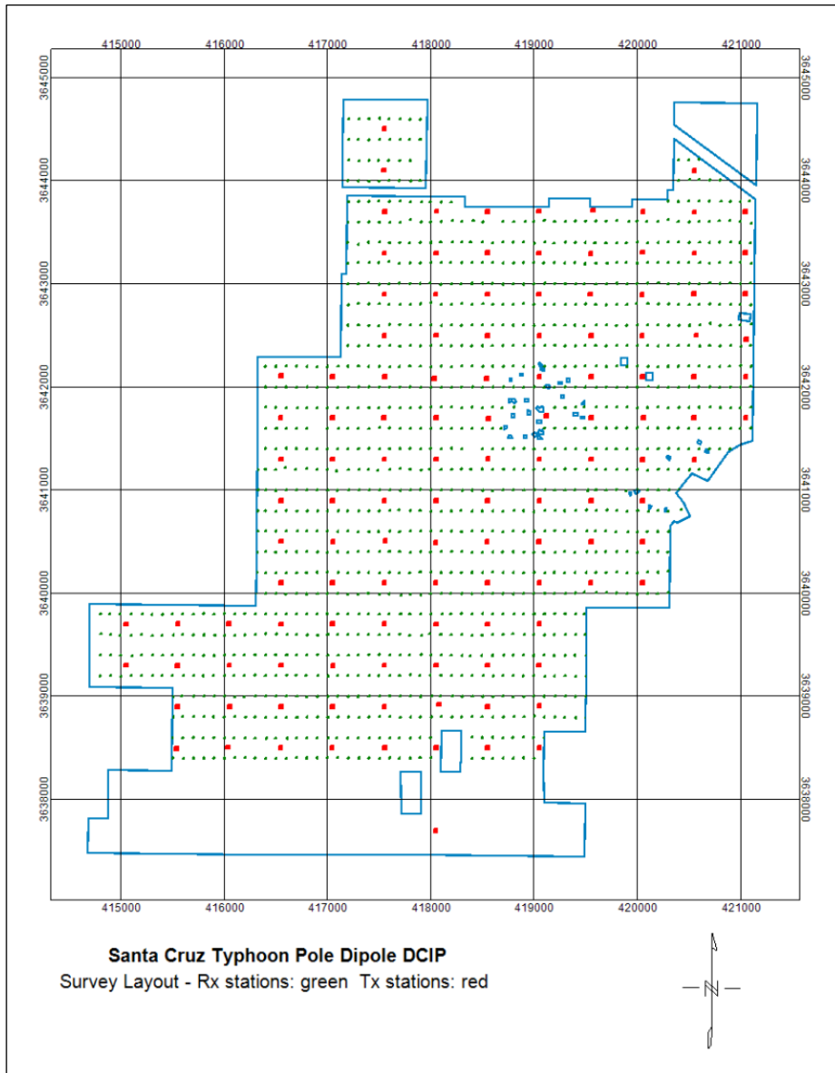
Figure 7-3: Layout of the Santa Cruz 3D IP Survey
