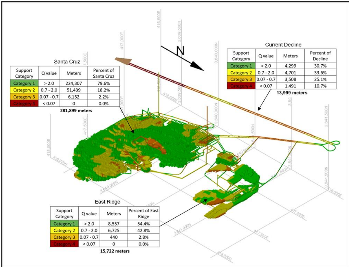
Figure 13-29: Isometric View of Most Recent Mine Design with Ground Support Estimates
