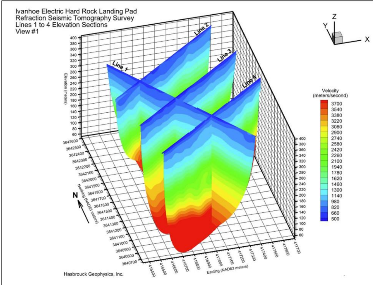
Figure 7-4: Refraction Seismic Tomography Survey Results
