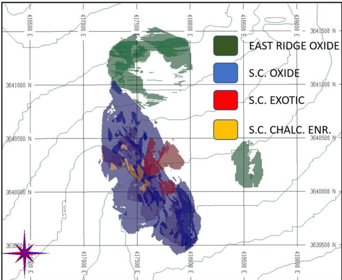
Figure 13-2: Plan View of Santa Cruz and East Ridge Mining Targets
