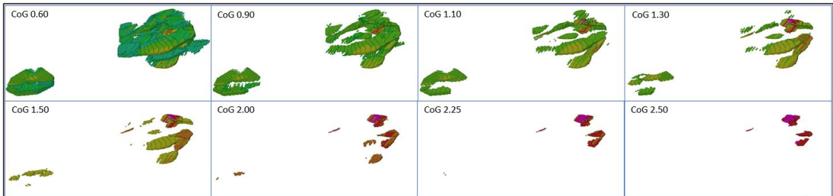
Figure 13-37: East Ridge Undiluted MSO Results (Looking to the West)
