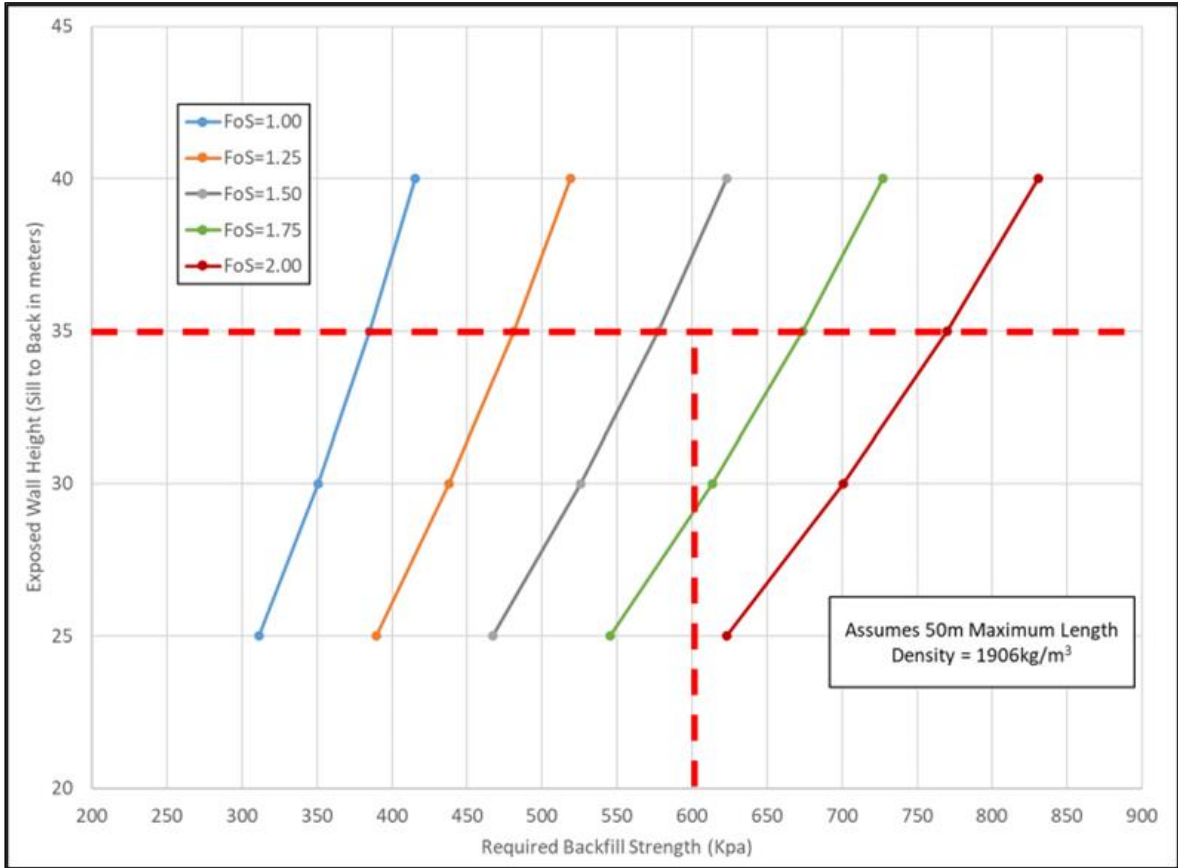
Figure 13-15: PBF Strength Estimates
