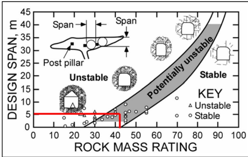
Figure 13-23: Critical Span Curve
