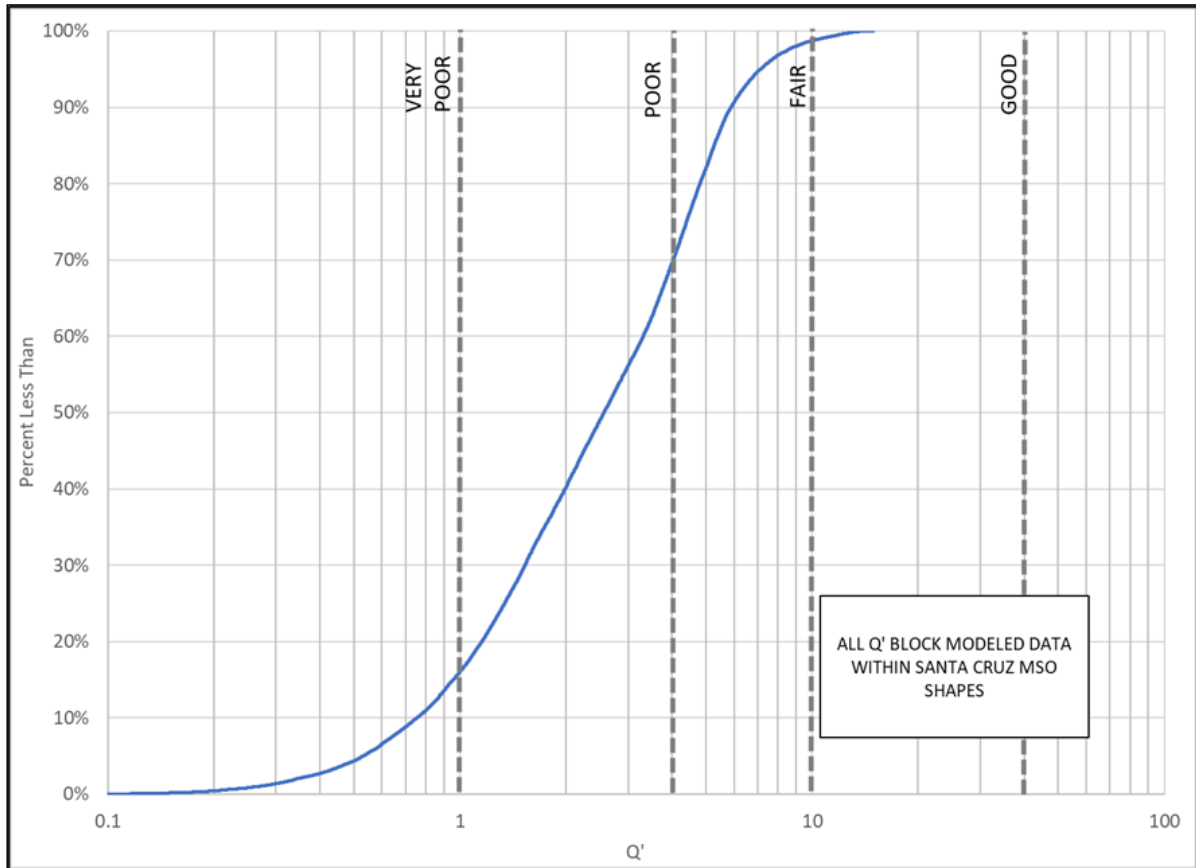
Figure 13-6: Cumulative Distribution Plot of All Q' Data within the Santa Cruz MSO Shapes
