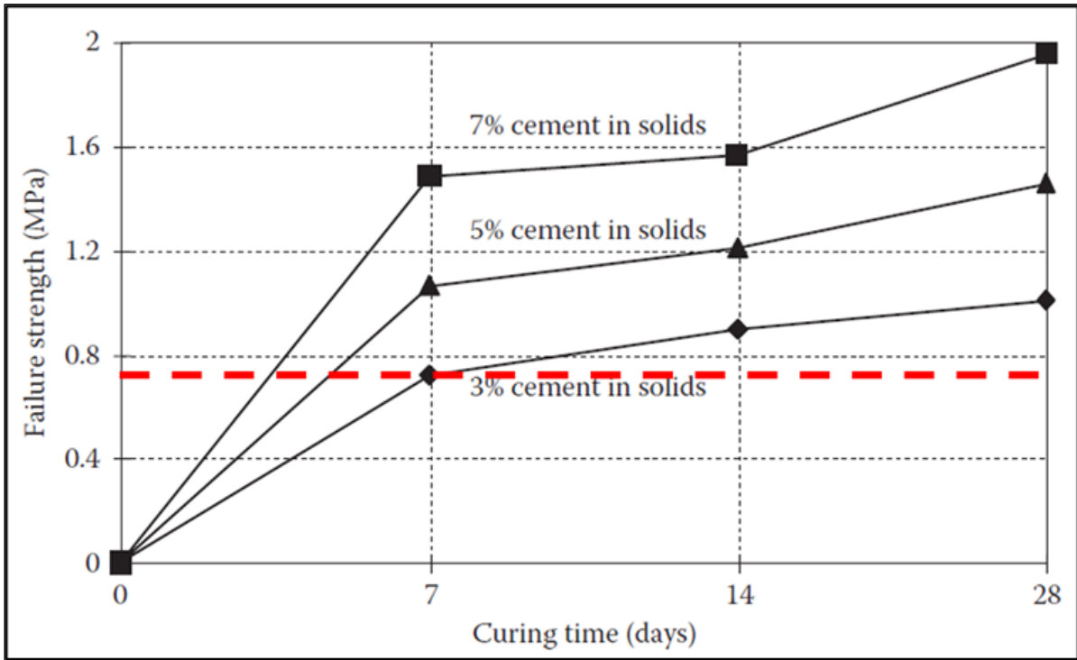
Figure 13-16: Cement in Solids Estimate
