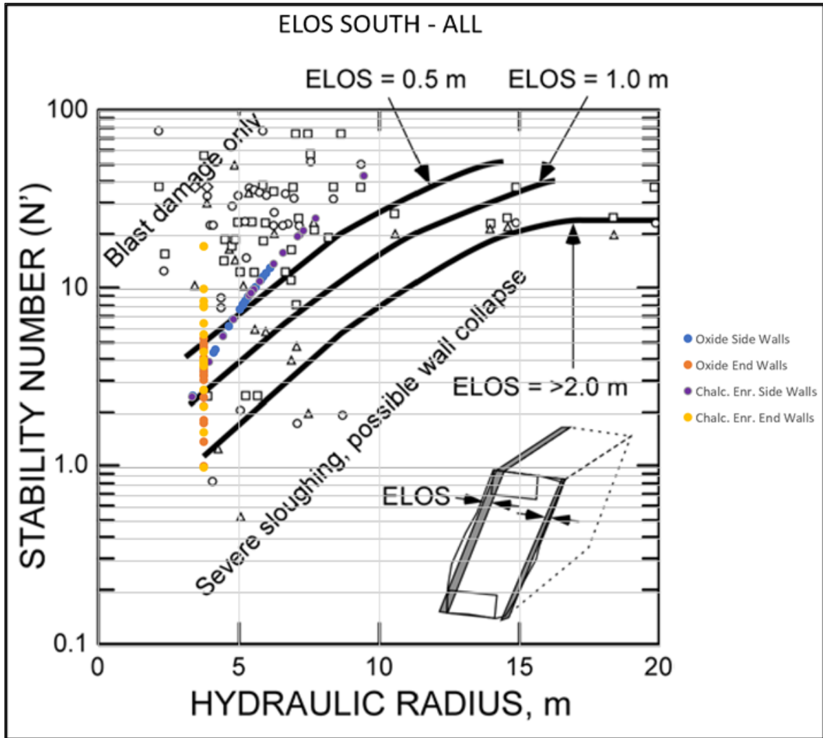
Figure 13-14: South Domain ELOS Estimates (10 m Wide, 30 m High)
