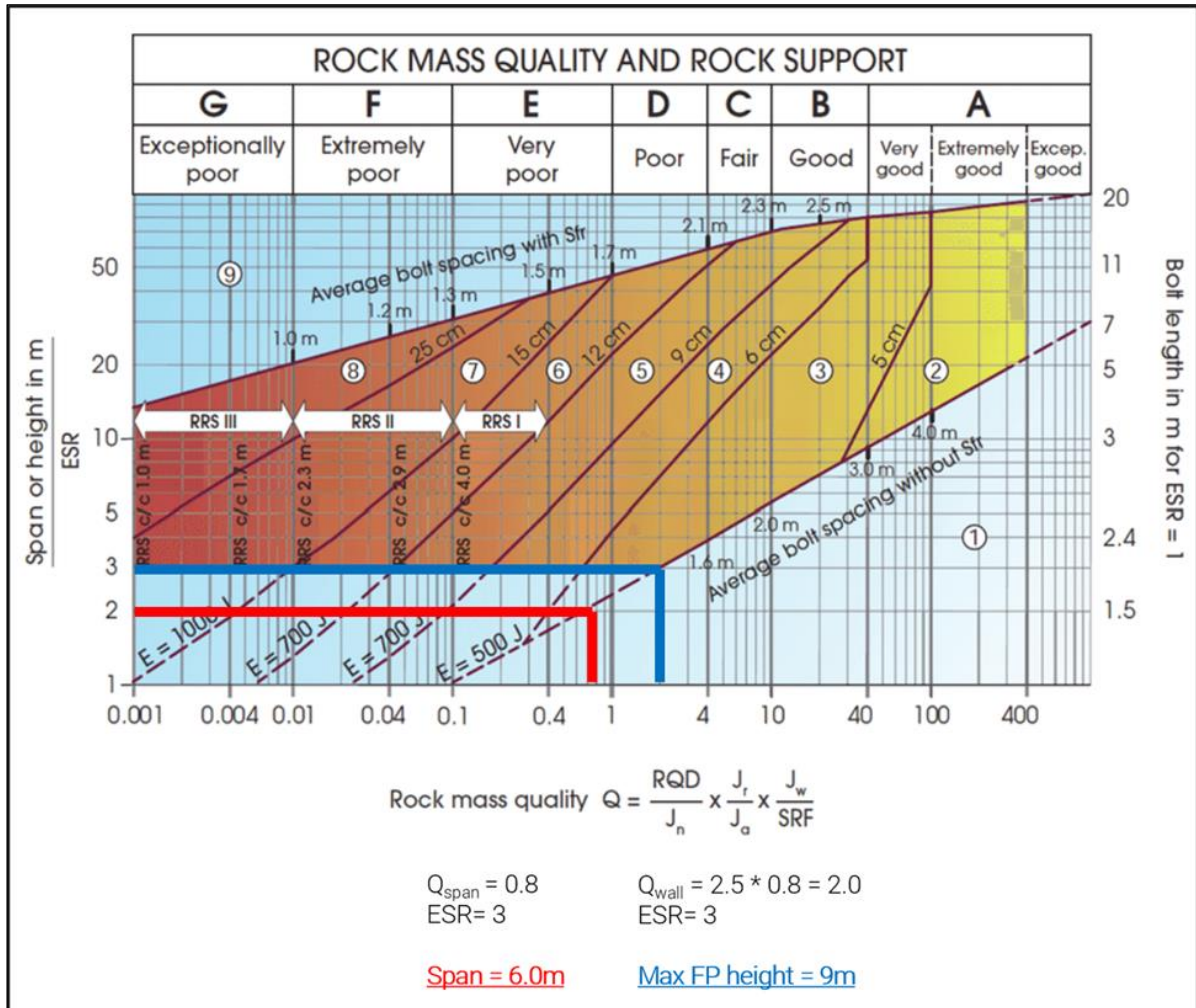
Figure 13-24: Ground Support Chart for DAF Span and Maximum Height
