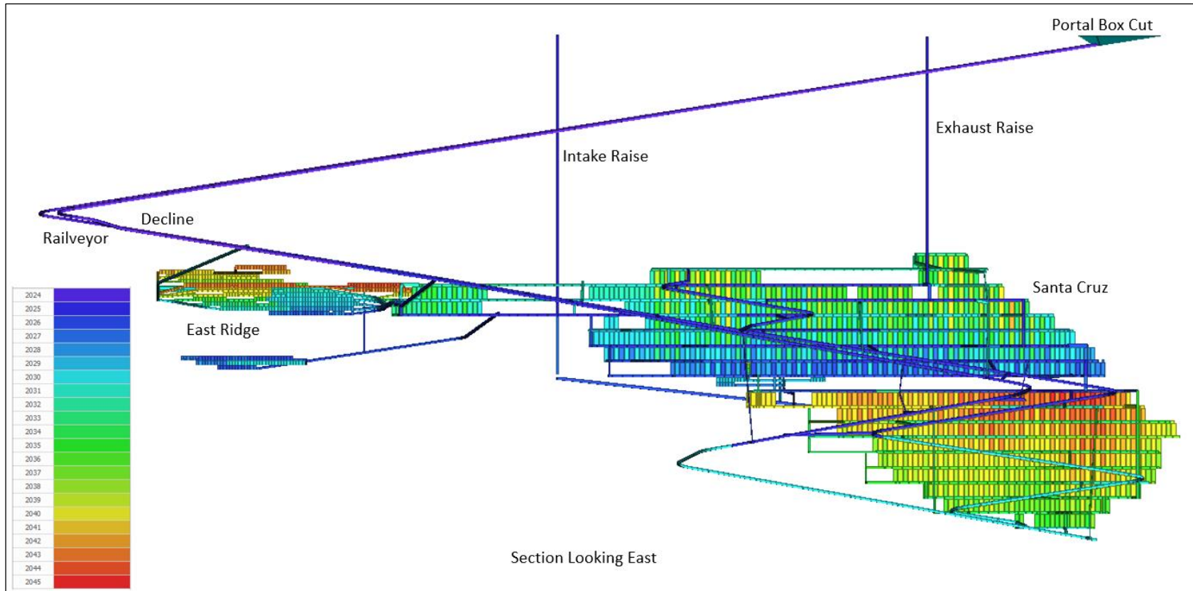
Figure 13-44: Mine Production Schedule Colored by Year (with Inferred)
