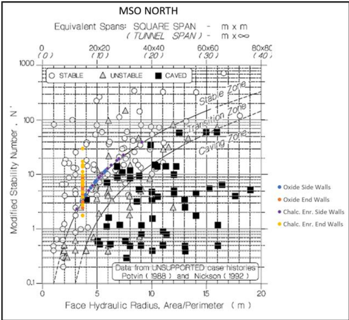
Figure 13-10: North Domain Stability Graph Results (10 m Wide, 30 m High)
